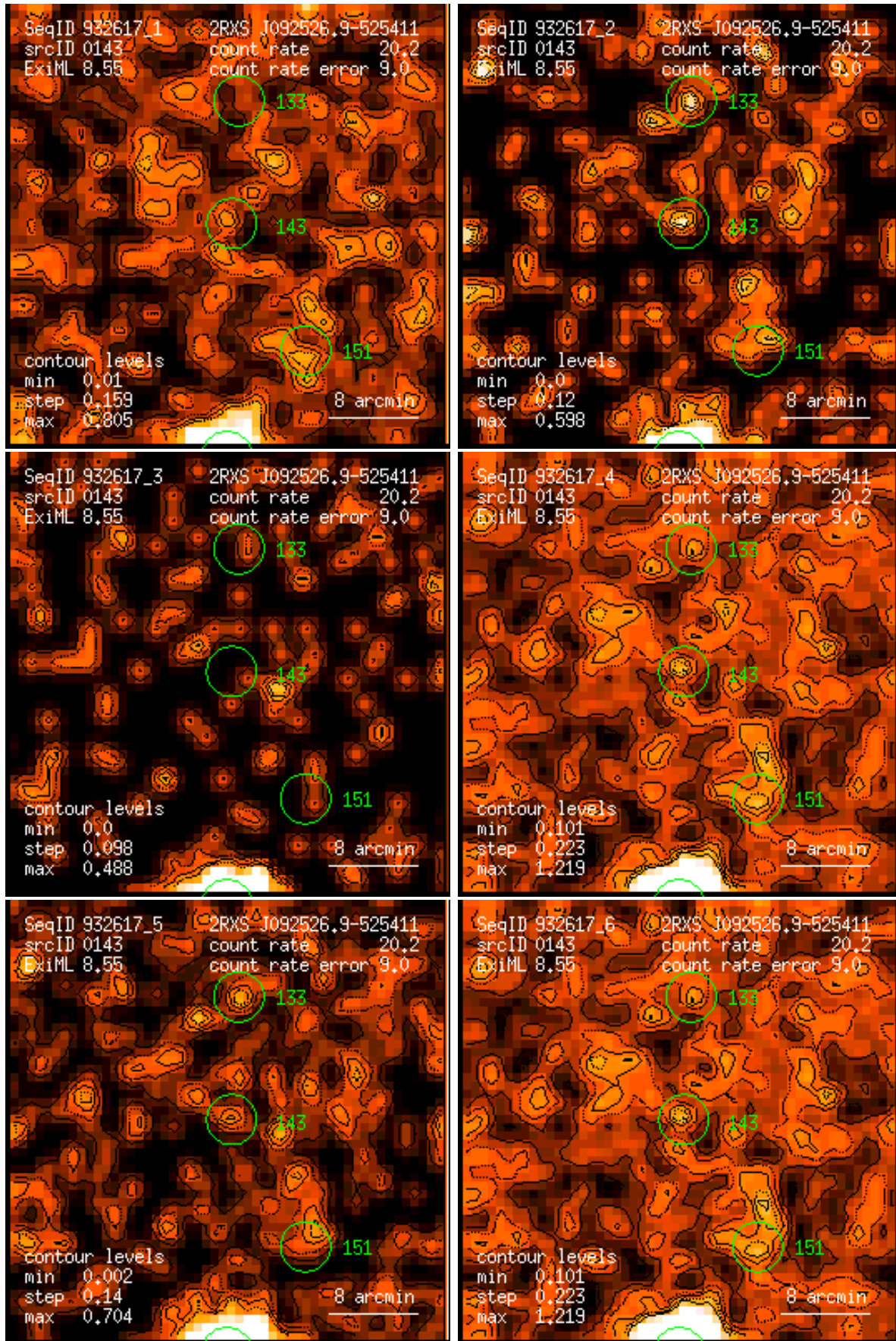
Figure 143: RASS 932617: detection 0143: band rate images, Gaussian filter: (1) PSPC channels 11 – 41, (2) 52 – 90, (3) 91 – 201, (4) 11 – 235, (5) 52 – 201, (6) 11 – 201. Broad band rates in counts/ks. Band rate contour levels in counts/ks/arcmin 2 .
