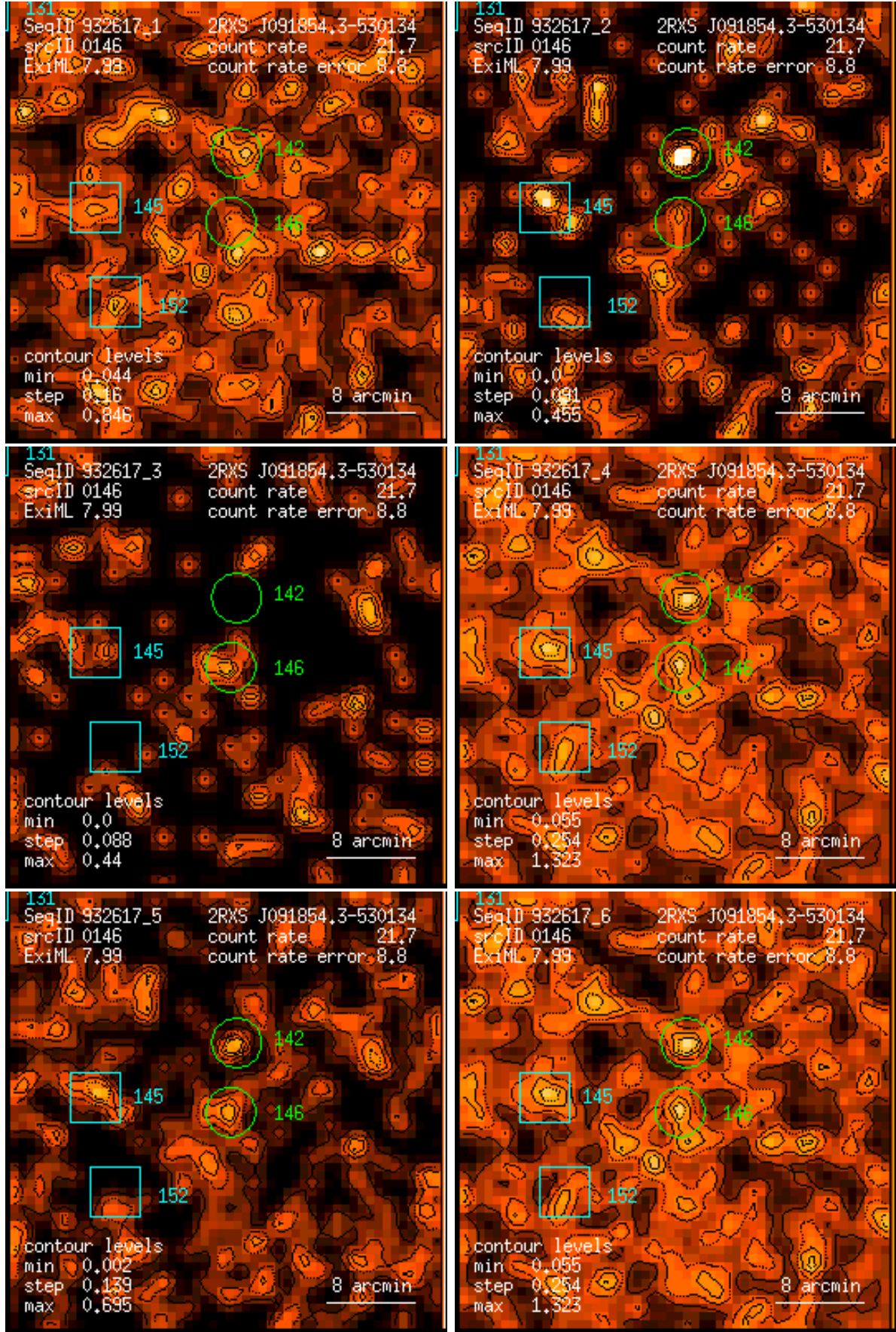
Figure 146: RASS 932617: detection 0146: band rate images, Gaussian filter: (1) PSPC channels 11 – 41, (2) 52 – 90, (3) 91 – 201, (4) 11 – 235, (5) 52 – 201, (6) 11 – 201. Broad band rates in counts/ks. Band rate contour levels in counts/ks/arcmin 2 .
