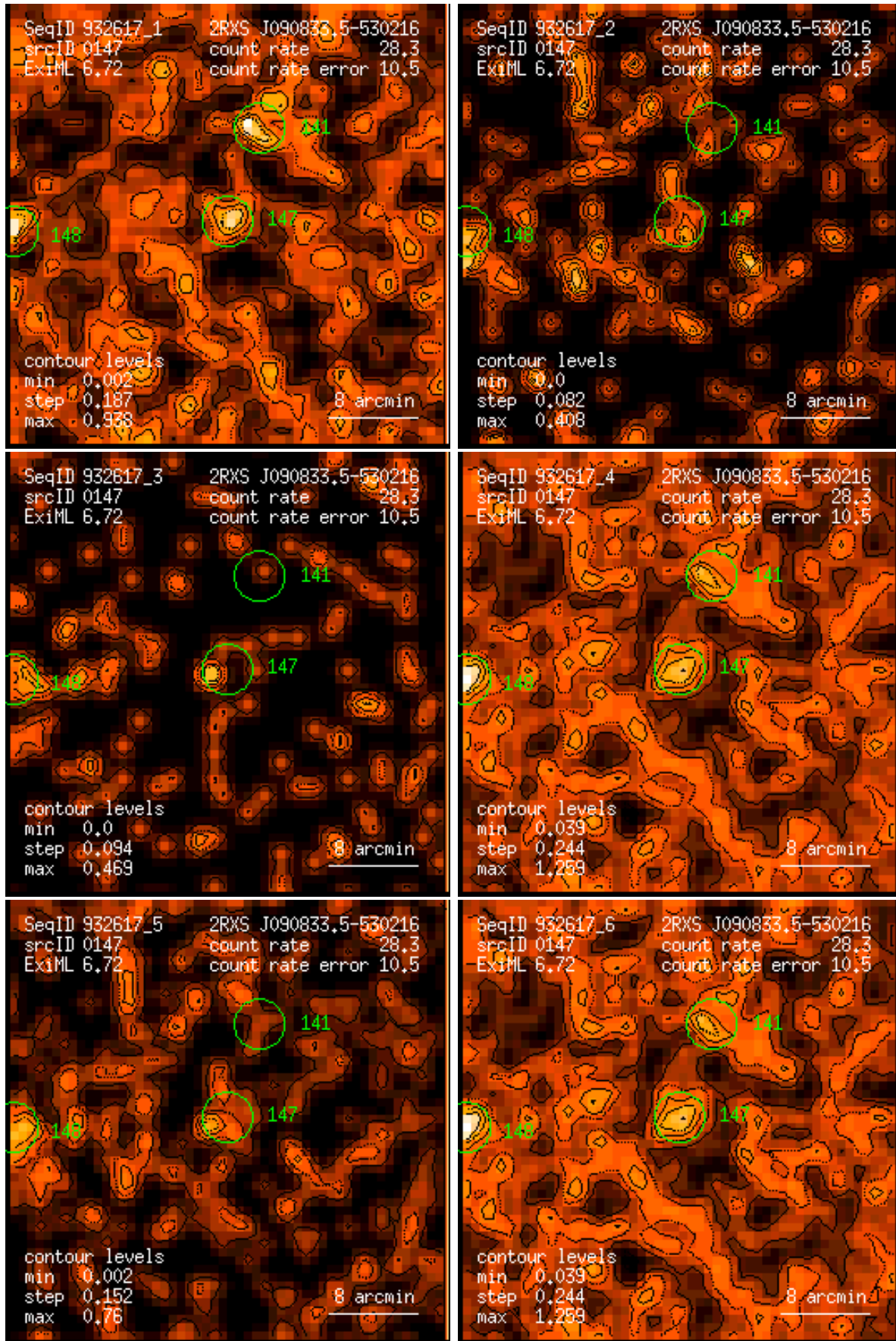
Figure 147: RASS 932617: detection 0147: band rate images, Gaussian filter: (1) PSPC channels 11 – 41, (2) 52 – 90, (3) 91 – 201, (4) 11 – 235, (5) 52 – 201, (6) 11 – 201. Broad band rates in counts/ks. Band rate contour levels in counts/ks/arcmin 2 .
