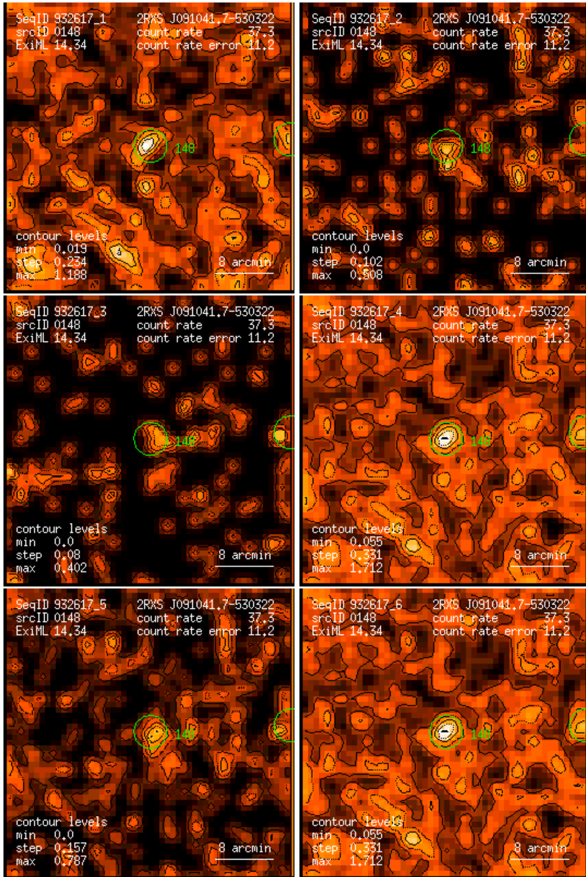
Figure 148: RASS 932617: detection 0148: band rate images, Gaussian filter: (1) PSPC channels 11 – 41, (2) 52 – 90, (3) 91 – 201, (4) 11 – 235, (5) 52 – 201, (6) 11 – 201. Broad band rates in counts/ks. Band rate contour levels in counts/ks/arcmin 2 .
