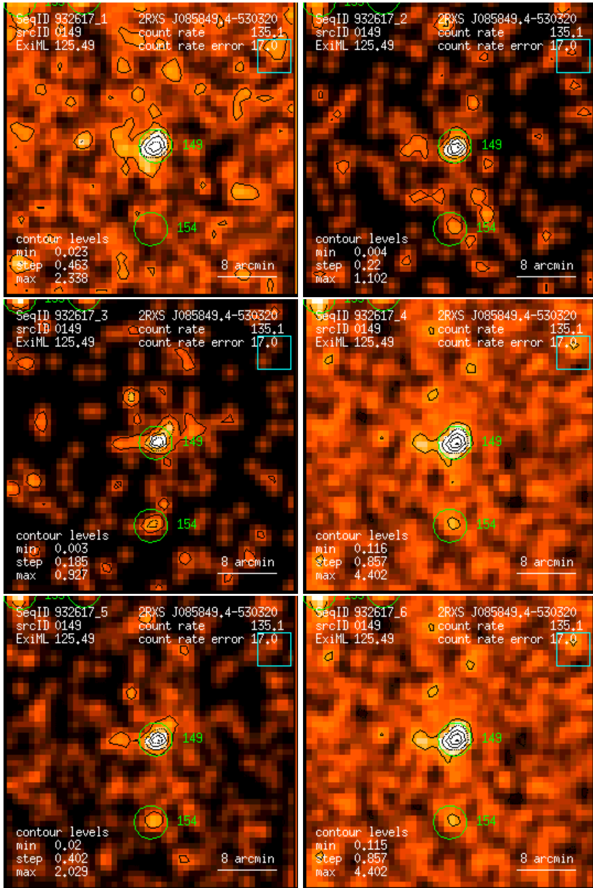
Figure 149: RASS 932617: detection 0149: band rate images, Gaussian filter: (1) PSPC channels 11 – 41, (2) 52 – 90, (3) 91 – 201, (4) 11 – 235, (5) 52 – 201, (6) 11 – 201. Broad band rates in counts/ks. Band rate contour levels in counts/ks/arcmin 2 .
