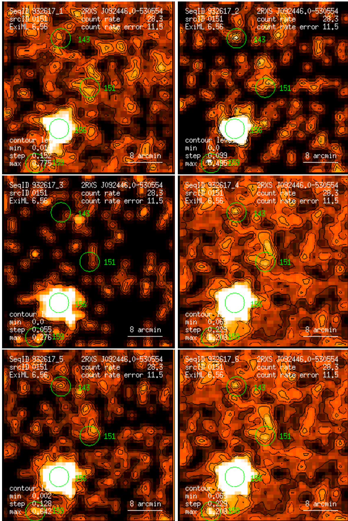
Figure 151: RASS 932617: detection 0151: band rate images, Gaussian filter: (1) PSPC channels 11 – 41, (2) 52 – 90, (3) 91 – 201, (4) 11 – 235, (5) 52 – 201, (6) 11 – 201. Broad band rates in counts/ks. Band rate contour levels in counts/ks/arcmin 2 .
