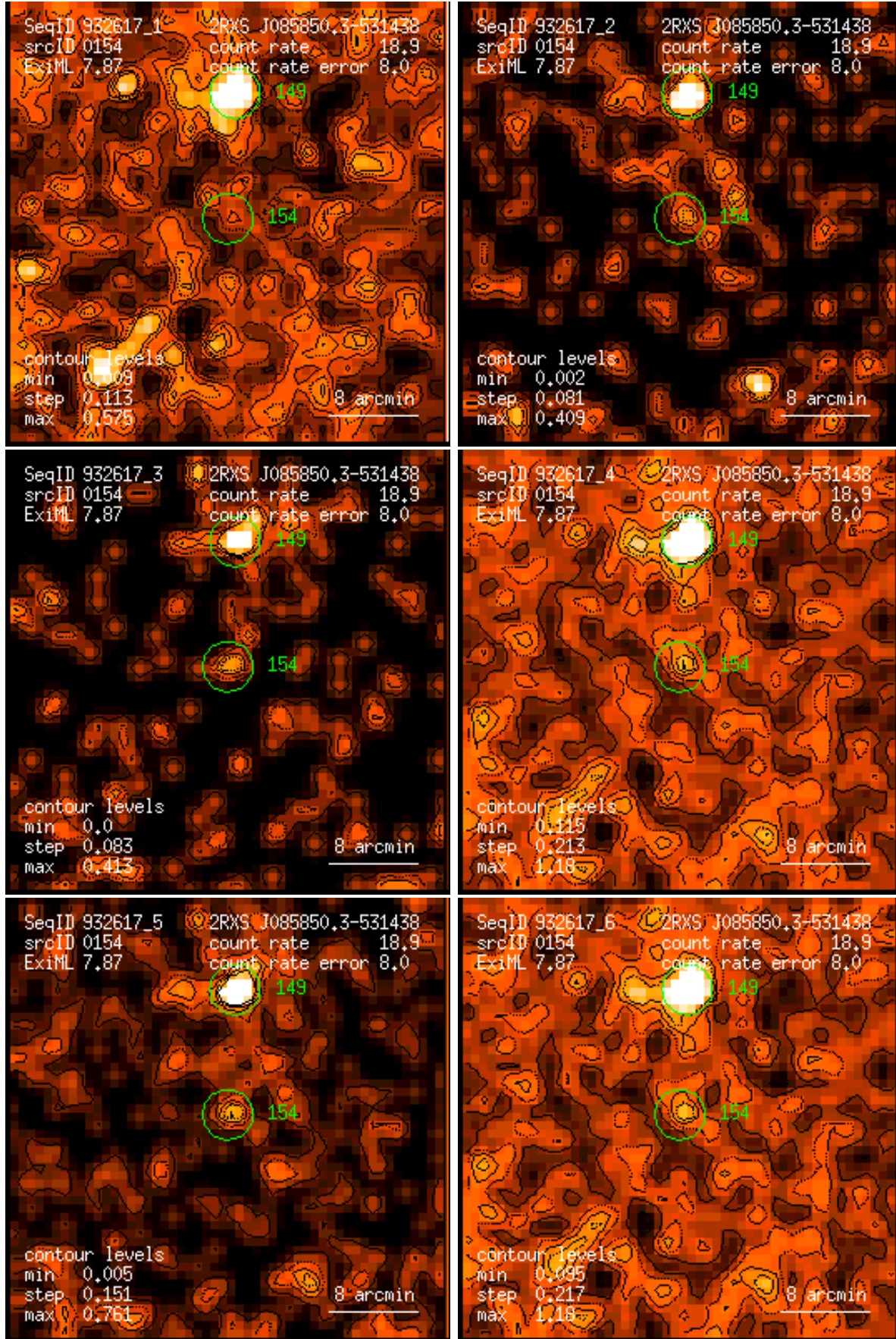
Figure 154: RASS 932617: detection 0154: band rate images, Gaussian filter: (1) PSPC channels 11 – 41, (2) 52 – 90, (3) 91 – 201, (4) 11 – 235, (5) 52 – 201, (6) 11 – 201. Broad band rates in counts/ks. Band rate contour levels in counts/ks/arcmin 2 .
