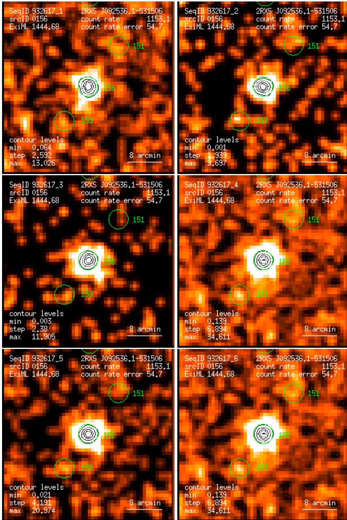
Figure 156: RASS 932617: detection 0156: band rate images, Gaussian filter: (1) PSPC channels 11 – 41, (2) 52 – 90, (3) 91 – 201, (4) 11 – 235, (5) 52 – 201, (6) 11 – 201. Broad band rates in counts/ks. Band rate contour levels in counts/ks/arcmin 2 .
