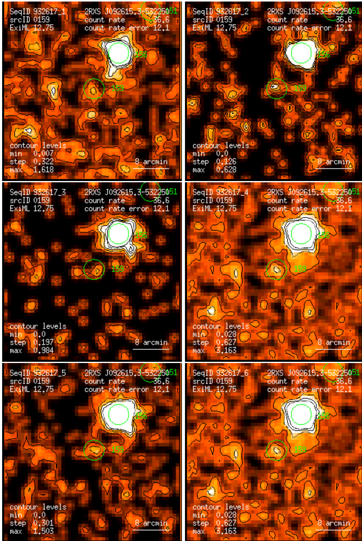
Figure 159: RASS 932617: detection 0159: band rate images, Gaussian filter: (1) PSPC channels 11 – 41, (2) 52 – 90, (3) 91 – 201, (4) 11 – 235, (5) 52 – 201, (6) 11 – 201. Broad band rates in counts/ks. Band rate contour levels in counts/ks/arcmin 2 .
