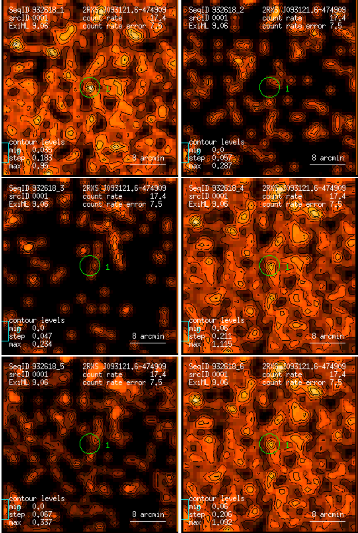
Figure 1: RASS 932618: detection 0001: band rate images, Gaussian filter: (1) PSPC channels 11 – 41, (2) 52 – 90, (3) 91 – 201, (4) 11 – 235, (5) 52 – 201, (6) 11 – 201. Broad band rates in counts/ks. Band rate contour levels in counts/ks/arcmin 2 .
