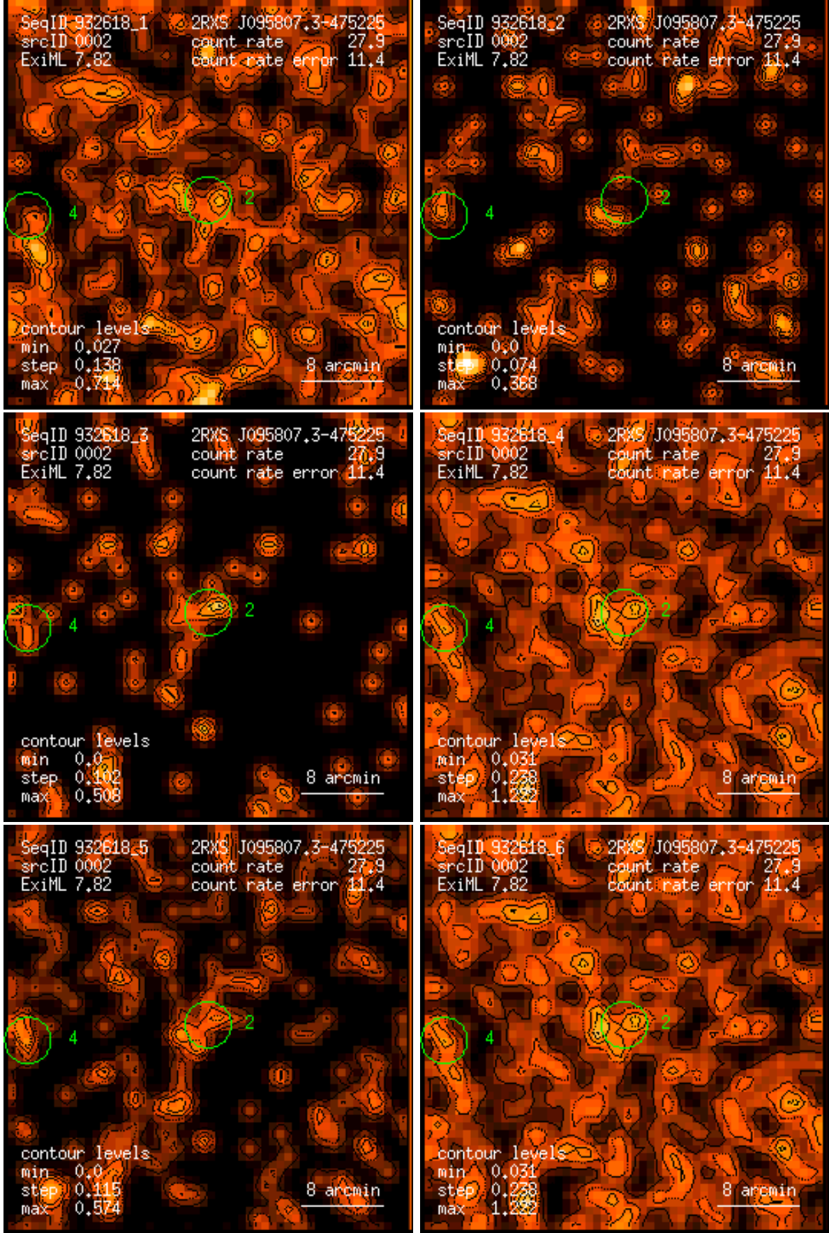
Figure 2: RASS 932618: detection 0002: band rate images, Gaussian filter: (1) PSPC channels 11 – 41, (2) 52 – 90, (3) 91 – 201, (4) 11 – 235, (5) 52 – 201, (6) 11 – 201. Broad band rates in counts/ks. Band rate contour levels in counts/ks/arcmin 2 .
