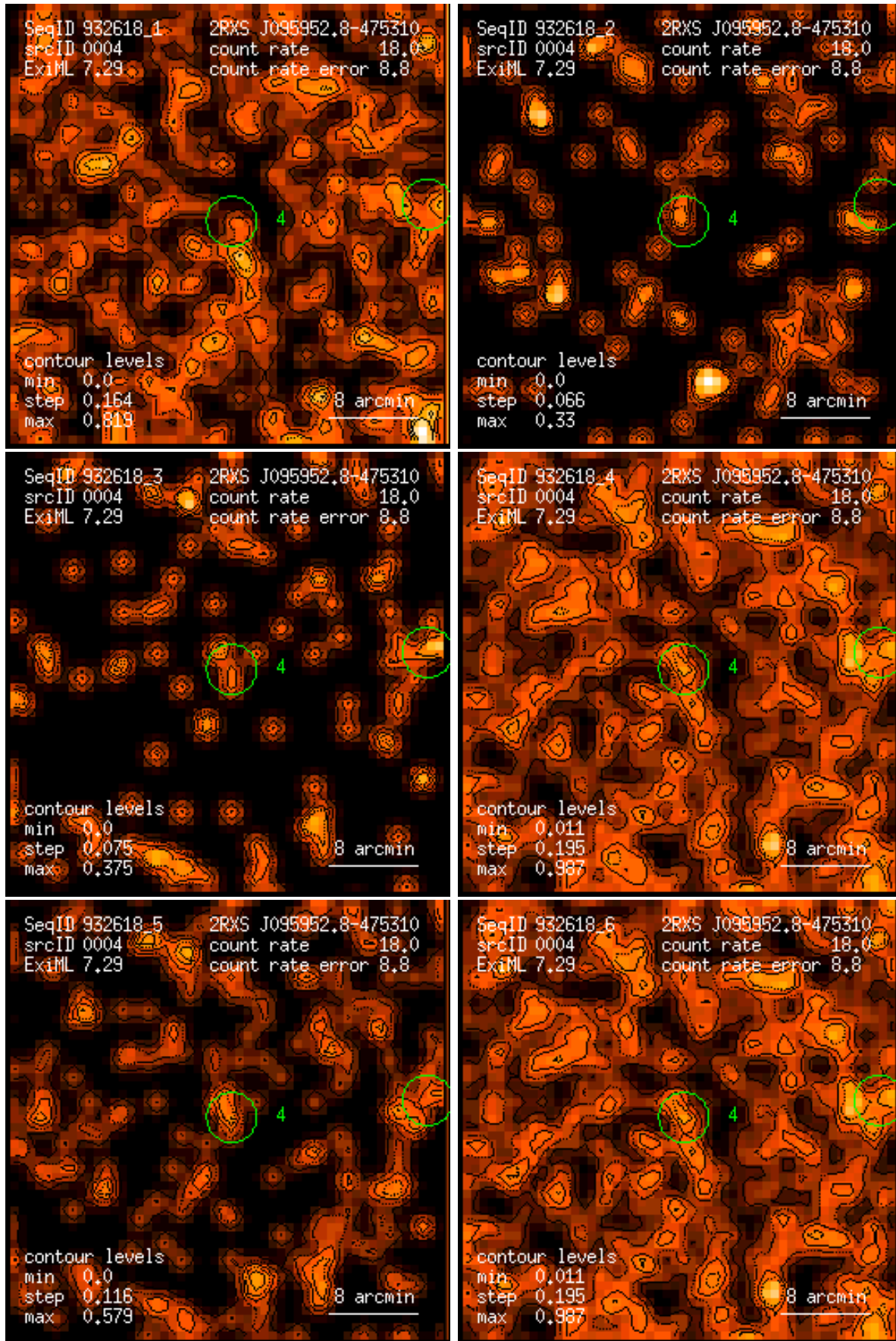
Figure 4: RASS 932618: detection 0004: band rate images, Gaussian filter: (1) PSPC channels 11 – 41, (2) 52 – 90, (3) 91 – 201, (4) 11 – 235, (5) 52 – 201, (6) 11 – 201. Broad band rates in counts/ks. Band rate contour levels in counts/ks/arcmin 2 .
