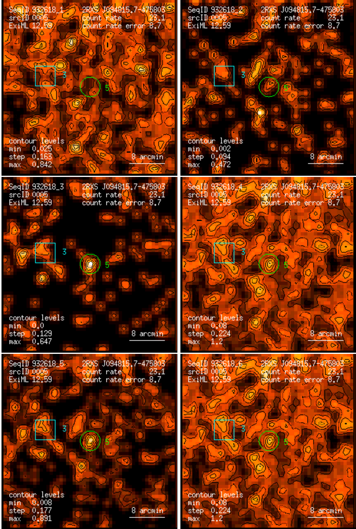
Figure 5: RASS 932618: detection 0005: band rate images, Gaussian filter: (1) PSPC channels 11 – 41, (2) 52 – 90, (3) 91 – 201, (4) 11 – 235, (5) 52 – 201, (6) 11 – 201. Broad band rates in counts/ks. Band rate contour levels in counts/ks/arcmin 2 .
