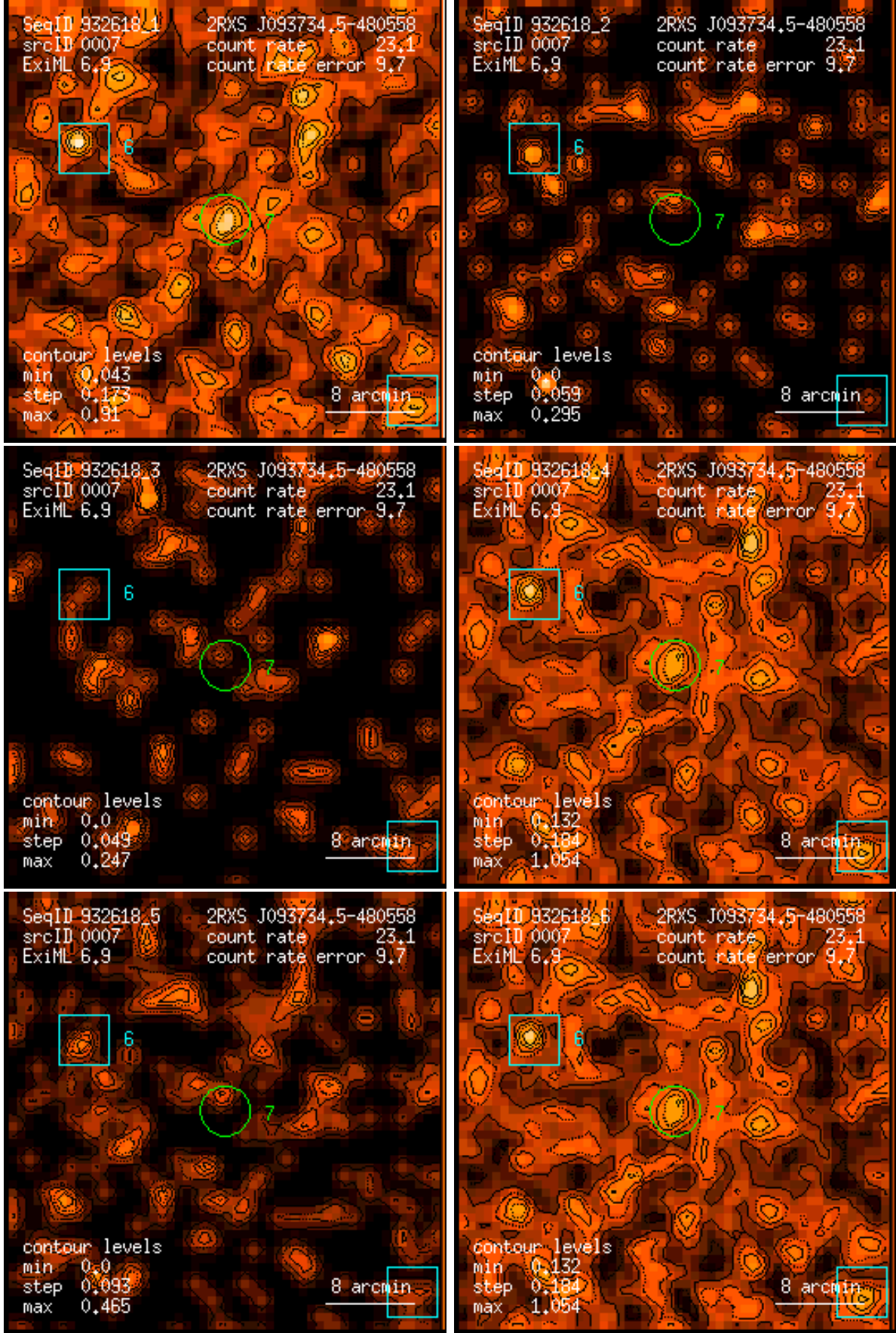
Figure 7: RASS 932618: detection 0007: band rate images, Gaussian filter: (1) PSPC channels 11 – 41, (2) 52 – 90, (3) 91 – 201, (4) 11 – 235, (5) 52 – 201, (6) 11 – 201. Broad band rates in counts/ks. Band rate contour levels in counts/ks/arcmin 2 .
