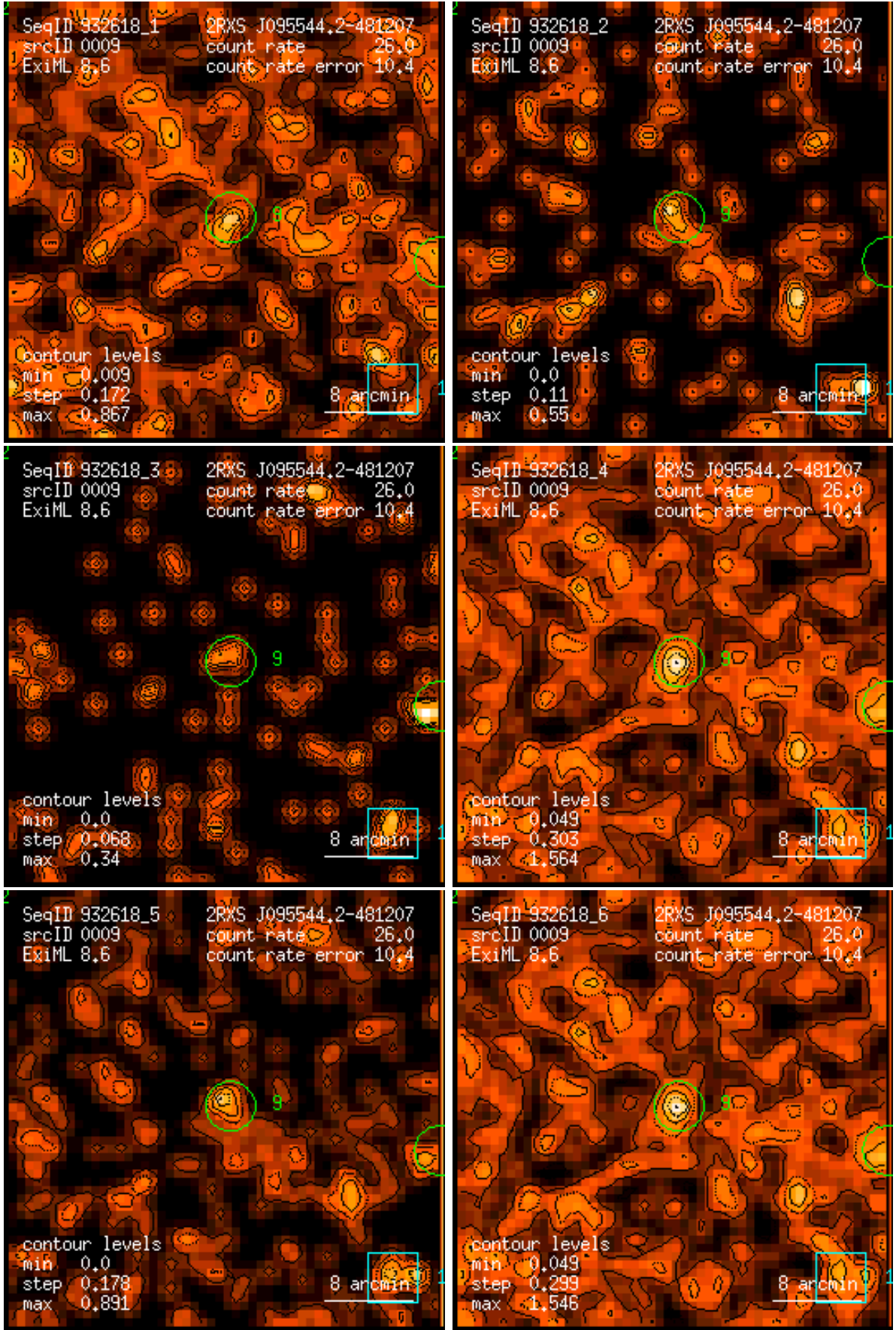
Figure 9: RASS 932618: detection 0009: band rate images, Gaussian filter: (1) PSPC channels 11 – 41, (2) 52 – 90, (3) 91 – 201, (4) 11 – 235, (5) 52 – 201, (6) 11 – 201. Broad band rates in counts/ks. Band rate contour levels in counts/ks/arcmin 2 .
