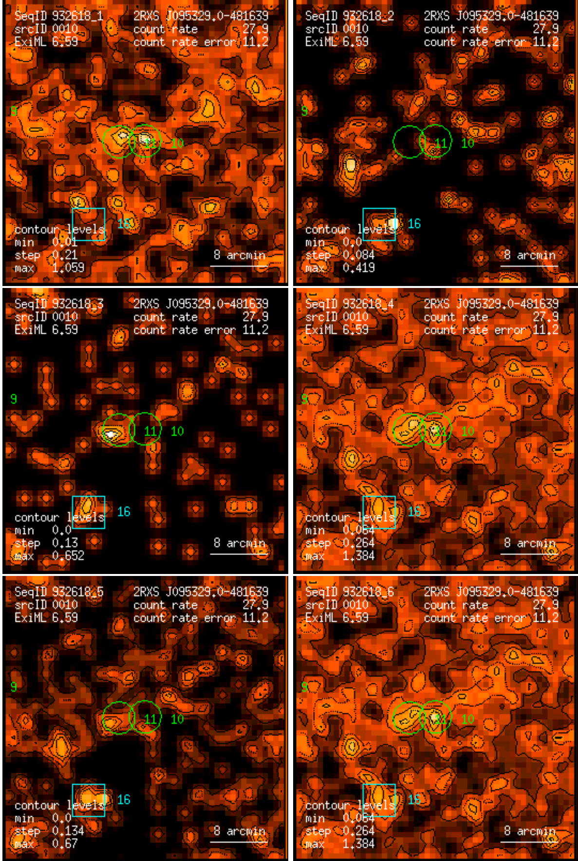
Figure 10: RASS 932618: detection 0010: band rate images, Gaussian filter: (1) PSPC channels 11 – 41, (2) 52 – 90, (3) 91 – 201, (4) 11 – 235, (5) 52 – 201, (6) 11 – 201. Broad band rates in counts/ks. Band rate contour levels in counts/ks/arcmin 2 .
