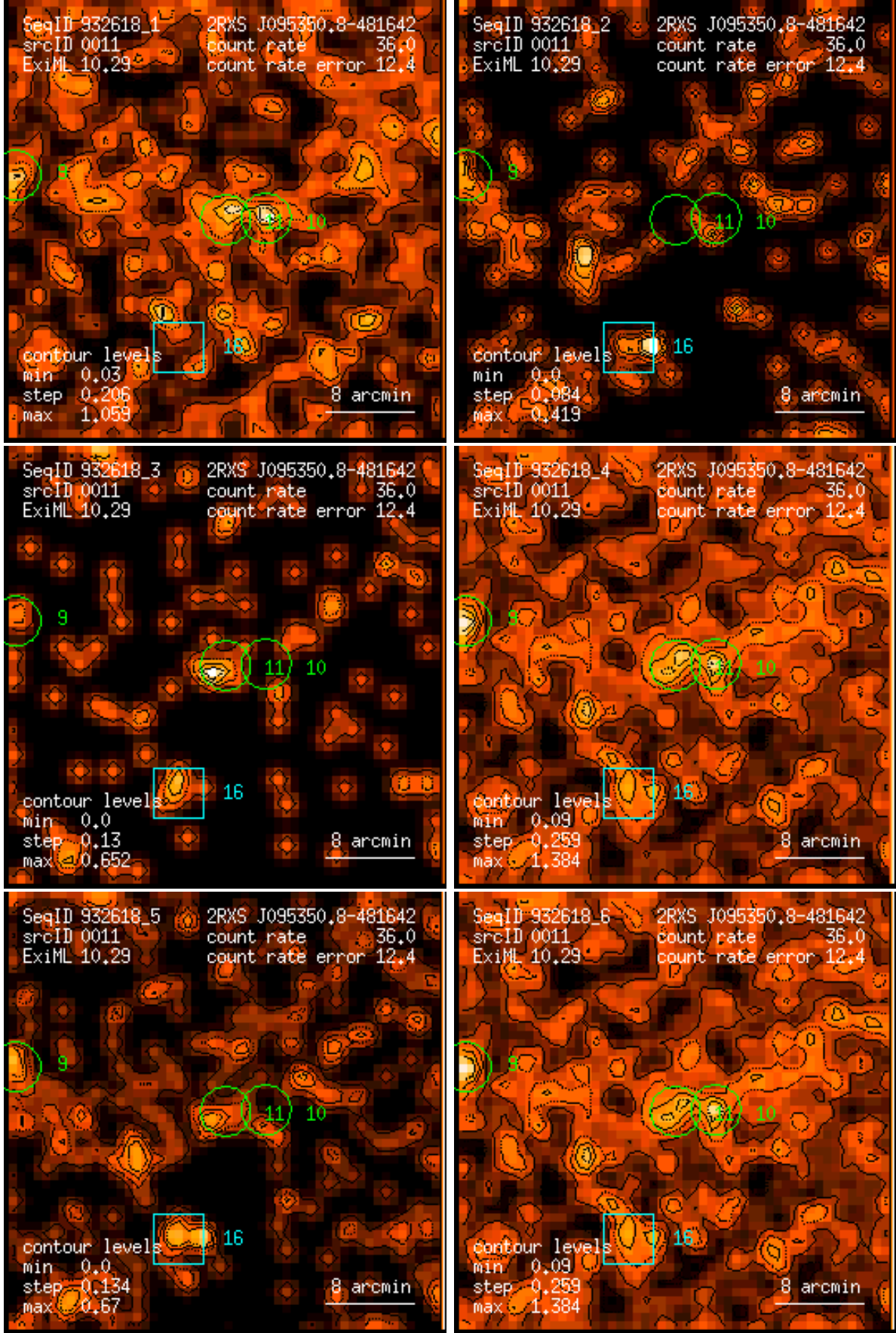
Figure 11: RASS 932618: detection 0011: band rate images, Gaussian filter: (1) PSPC channels 11 – 41, (2) 52 – 90, (3) 91 – 201, (4) 11 – 235, (5) 52 – 201, (6) 11 – 201. Broad band rates in counts/ks. Band rate contour levels in counts/ks/arcmin 2 .
