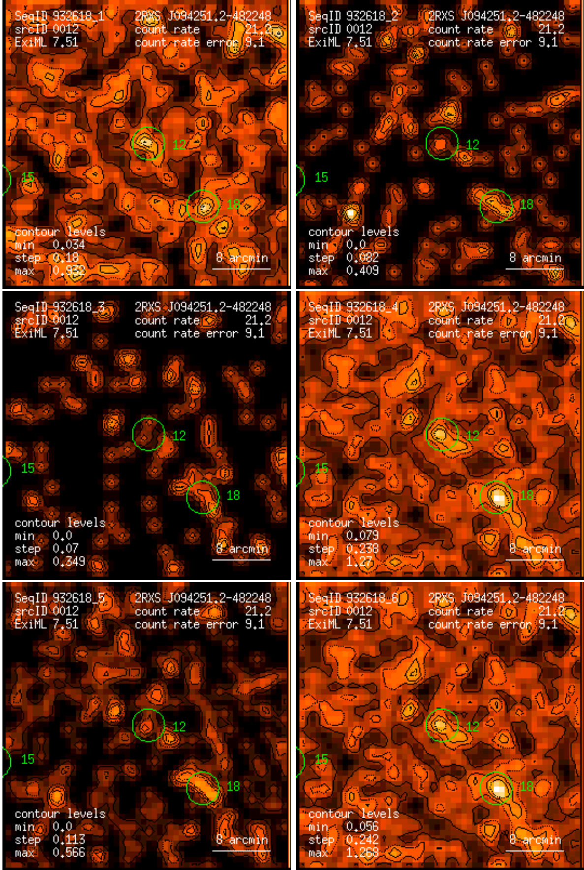
Figure 12: RASS 932618: detection 0012: band rate images, Gaussian filter: (1) PSPC channels 11 – 41, (2) 52 – 90, (3) 91 – 201, (4) 11 – 235, (5) 52 – 201, (6) 11 – 201. Broad band rates in counts/ks. Band rate contour levels in counts/ks/arcmin 2 .
