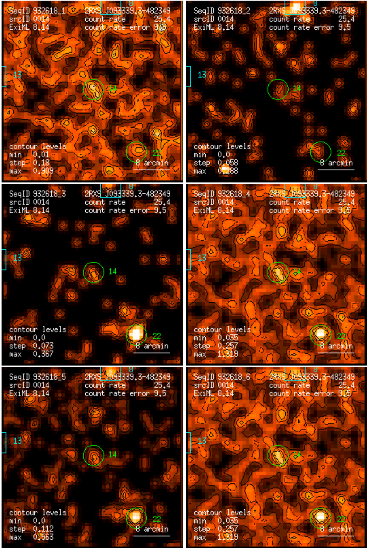
Figure 14: RASS 932618: detection 0014: band rate images, Gaussian filter: (1) PSPC channels 11 – 41, (2) 52 – 90, (3) 91 – 201, (4) 11 – 235, (5) 52 – 201, (6) 11 – 201. Broad band rates in counts/ks. Band rate contour levels in counts/ks/arcmin 2 .
