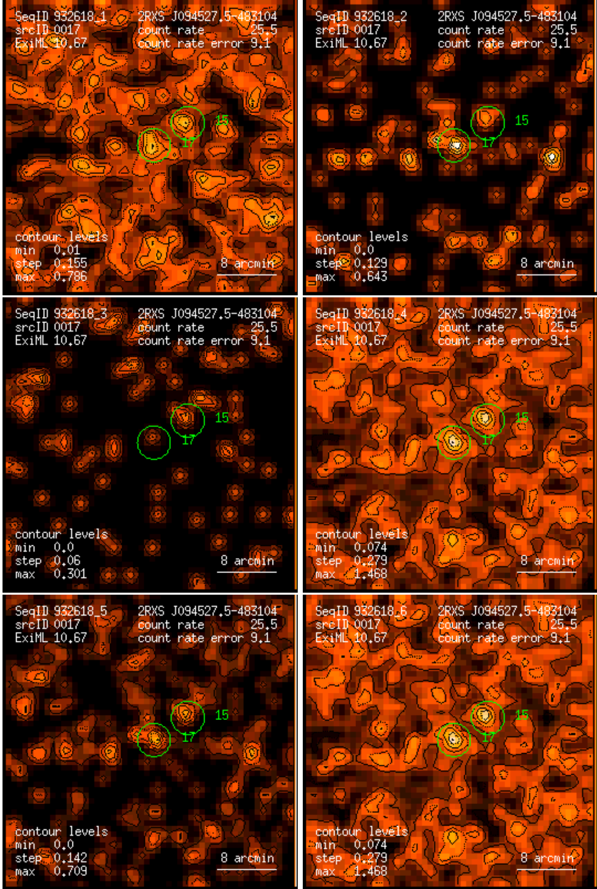
Figure 17: RASS 932618: detection 0017: band rate images, Gaussian filter: (1) PSPC channels 11 – 41, (2) 52 – 90, (3) 91 – 201, (4) 11 – 235, (5) 52 – 201, (6) 11 – 201. Broad band rates in counts/ks. Band rate contour levels in counts/ks/arcmin 2 .
