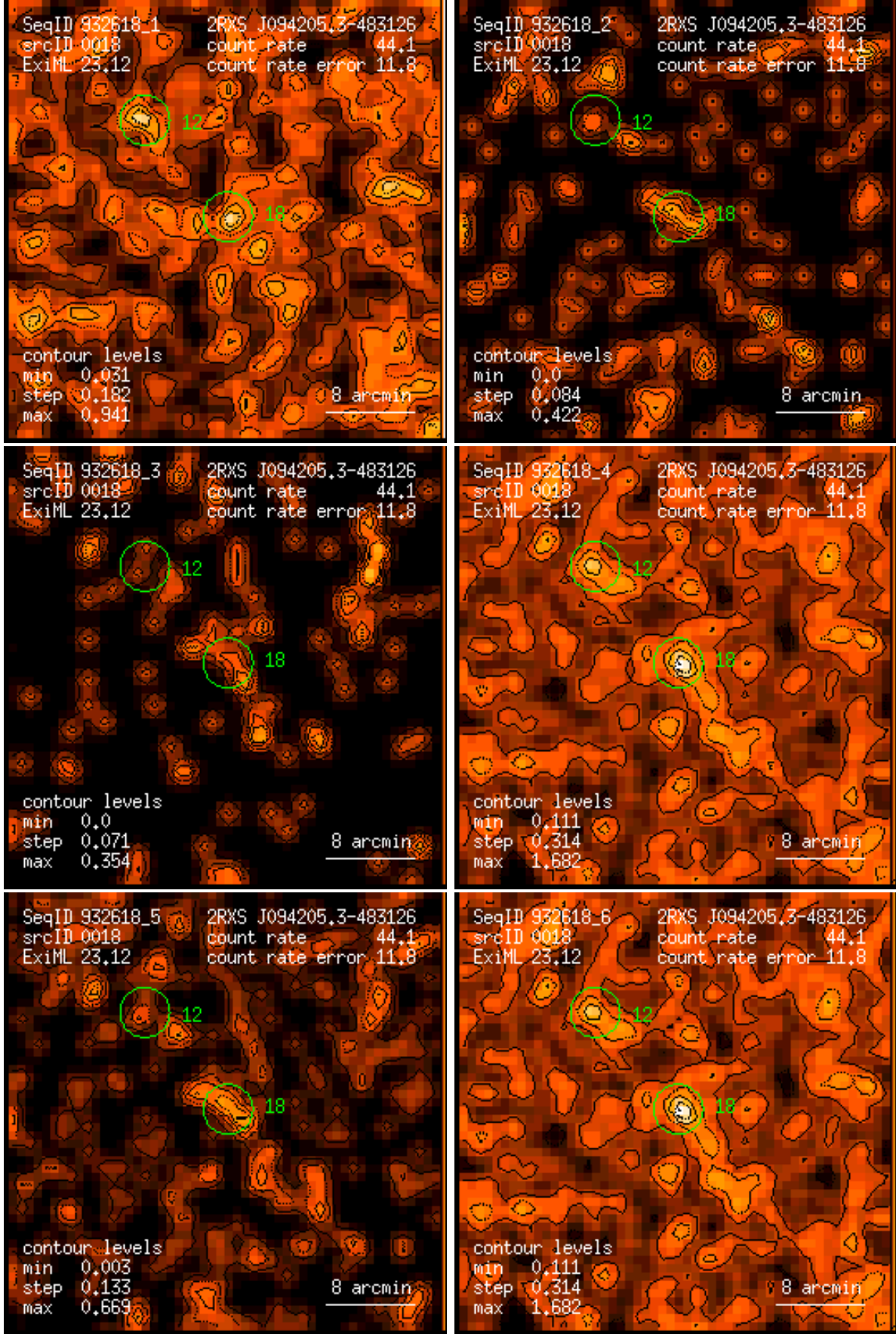
Figure 18: RASS 932618: detection 0018: band rate images, Gaussian filter: (1) PSPC channels 11 – 41, (2) 52 – 90, (3) 91 – 201, (4) 11 – 235, (5) 52 – 201, (6) 11 – 201. Broad band rates in counts/ks. Band rate contour levels in counts/ks/arcmin 2 .
