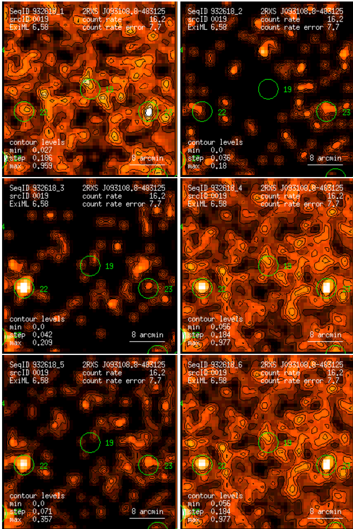
Figure 19: RASS 932618: detection 0019: band rate images, Gaussian filter: (1) PSPC channels 11 – 41, (2) 52 – 90, (3) 91 – 201, (4) 11 – 235, (5) 52 – 201, (6) 11 – 201. Broad band rates in counts/ks. Band rate contour levels in counts/ks/arcmin 2 .
