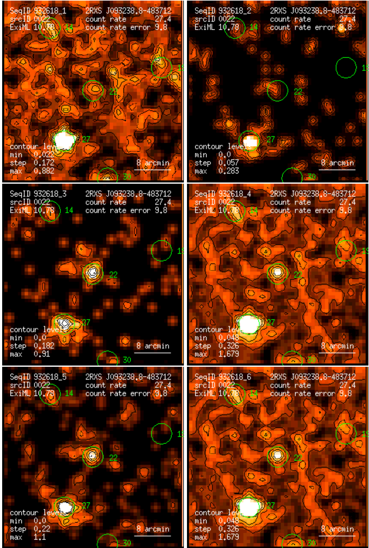
Figure 22: RASS 932618: detection 0022: band rate images, Gaussian filter: (1) PSPC channels 11 – 41, (2) 52 – 90, (3) 91 – 201, (4) 11 – 235, (5) 52 – 201, (6) 11 – 201. Broad band rates in counts/ks. Band rate contour levels in counts/ks/arcmin 2 .
