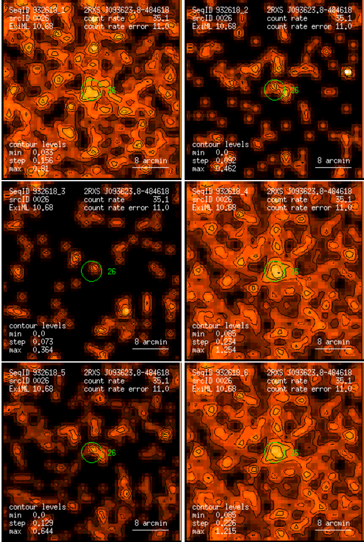
Figure 26: RASS 932618: detection 0026: band rate images, Gaussian filter: (1) PSPC channels 11 – 41, (2) 52 – 90, (3) 91 – 201, (4) 11 – 235, (5) 52 – 201, (6) 11 – 201. Broad band rates in counts/ks. Band rate contour levels in counts/ks/arcmin 2 .
