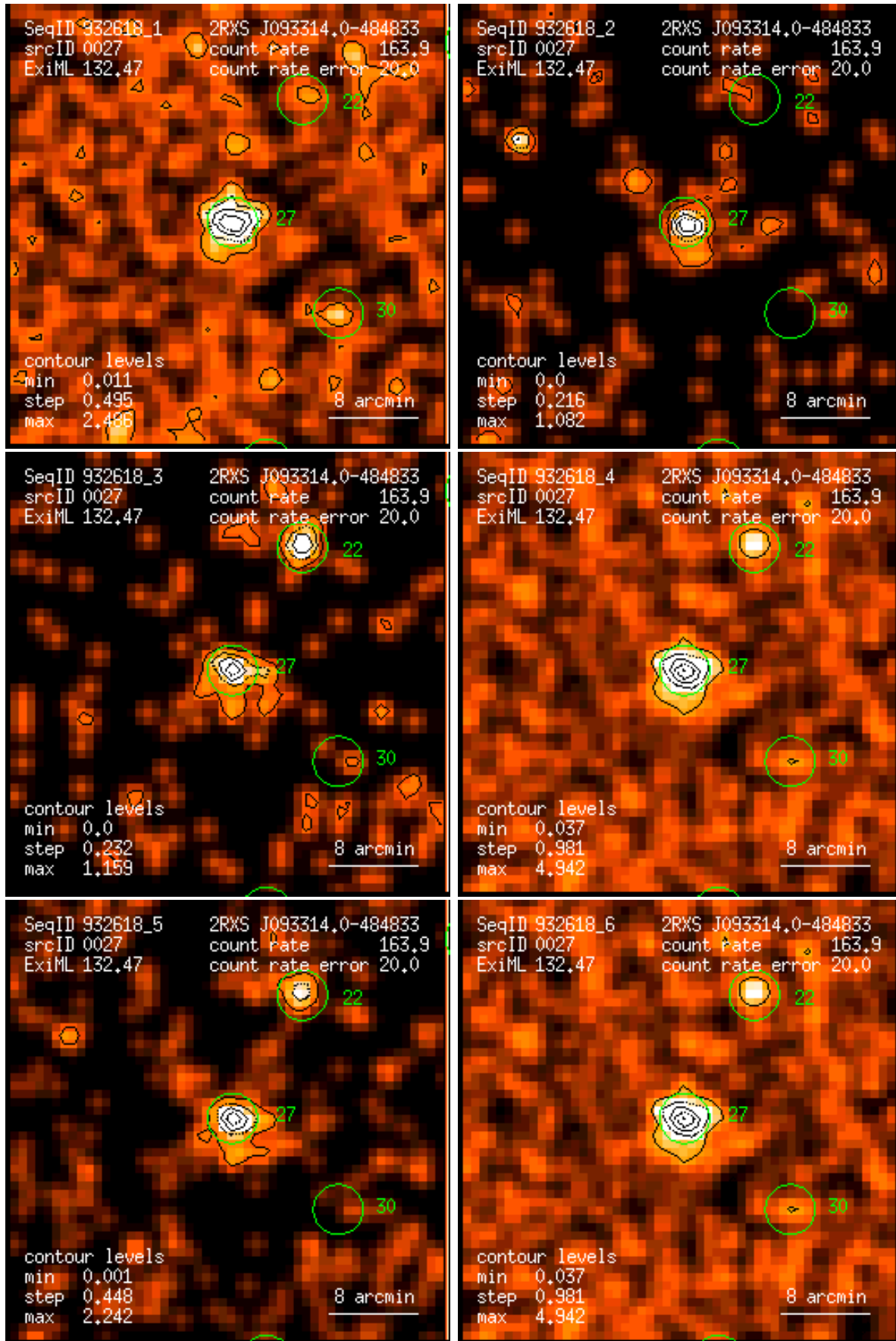
Figure 27: RASS 932618: detection 0027: band rate images, Gaussian filter: (1) PSPC channels 11 – 41, (2) 52 – 90, (3) 91 – 201, (4) 11 – 235, (5) 52 – 201, (6) 11 – 201. Broad band rates in counts/ks. Band rate contour levels in counts/ks/arcmin 2 .
