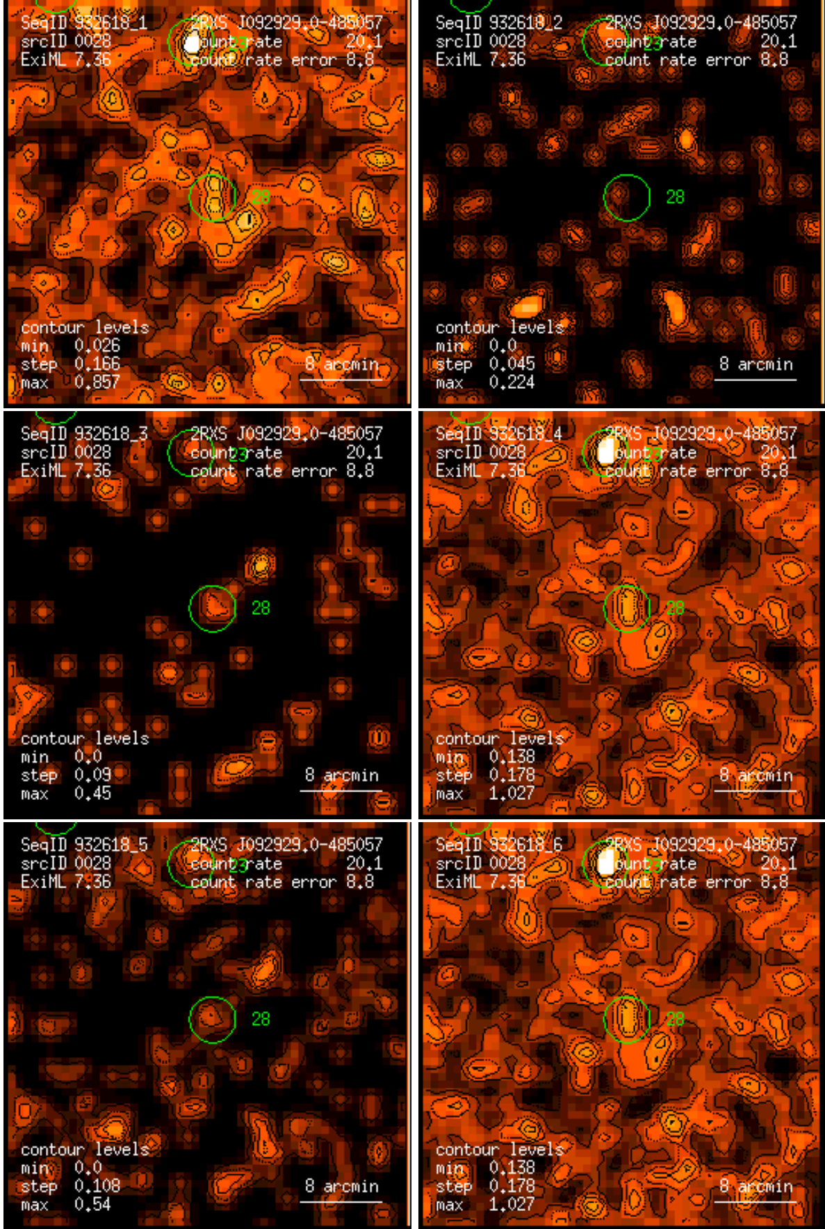
Figure 28: RASS 932618: detection 0028: band rate images, Gaussian filter: (1) PSPC channels 11 – 41, (2) 52 – 90, (3) 91 – 201, (4) 11 – 235, (5) 52 – 201, (6) 11 – 201. Broad band rates in counts/ks. Band rate contour levels in counts/ks/arcmin 2 .
