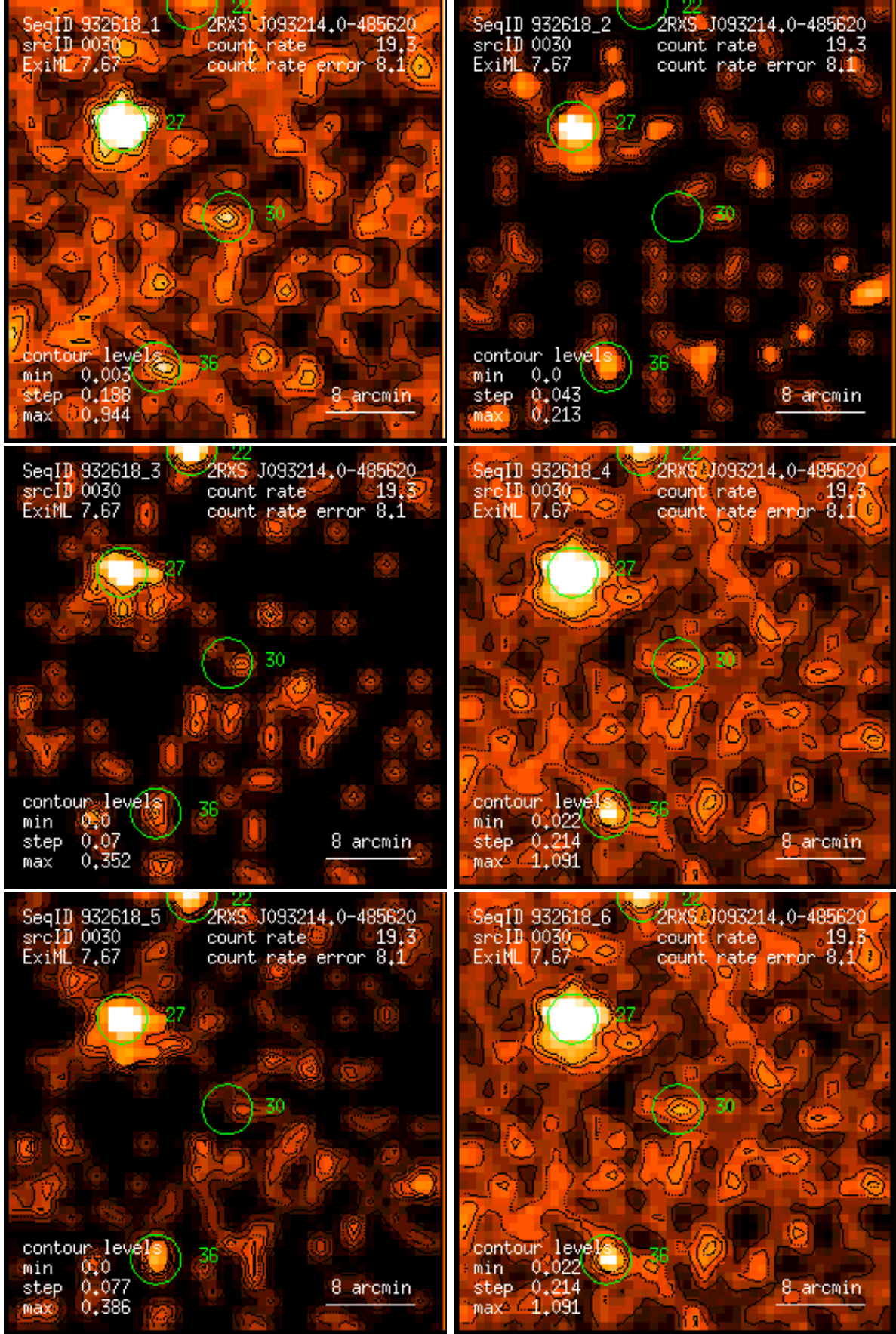
Figure 30: RASS 932618: detection 0030: band rate images, Gaussian filter: (1) PSPC channels 11 – 41, (2) 52 – 90, (3) 91 – 201, (4) 11 – 235, (5) 52 – 201, (6) 11 – 201. Broad band rates in counts/ks. Band rate contour levels in counts/ks/arcmin 2 .
