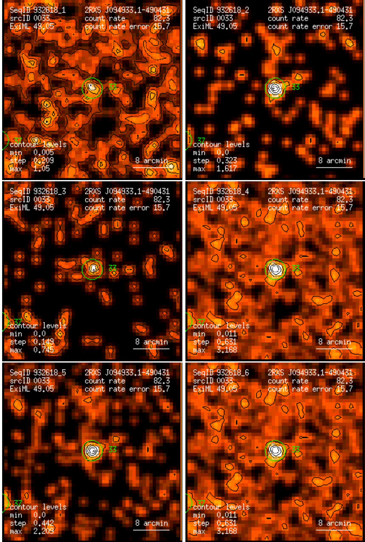
Figure 33: RASS 932618: detection 0033: band rate images, Gaussian filter: (1) PSPC channels 11 – 41, (2) 52 – 90, (3) 91 – 201, (4) 11 – 235, (5) 52 – 201, (6) 11 – 201. Broad band rates in counts/ks. Band rate contour levels in counts/ks/arcmin 2 .
