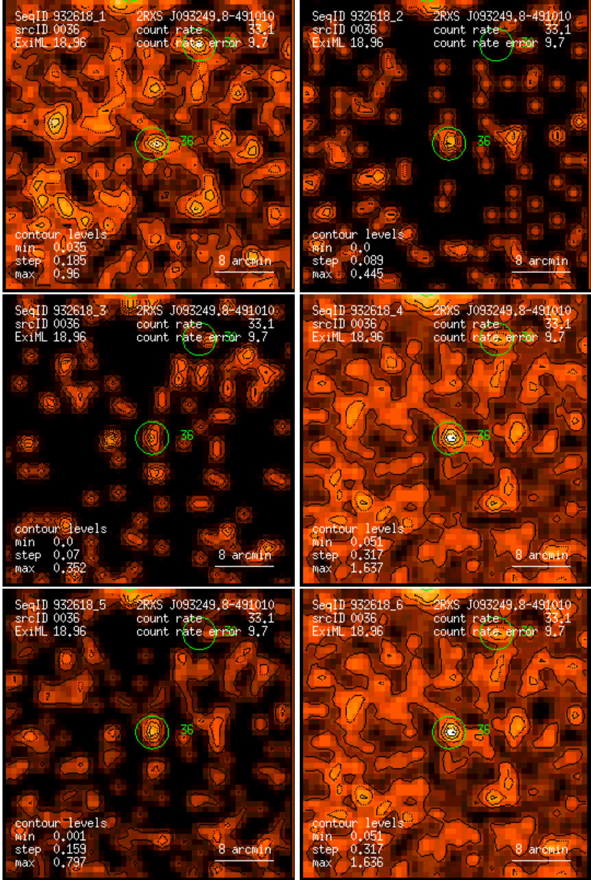
Figure 36: RASS 932618: detection 0036: band rate images, Gaussian filter: (1) PSPC channels 11 – 41, (2) 52 – 90, (3) 91 – 201, (4) 11 – 235, (5) 52 – 201, (6) 11 – 201. Broad band rates in counts/ks. Band rate contour levels in counts/ks/arcmin 2 .
