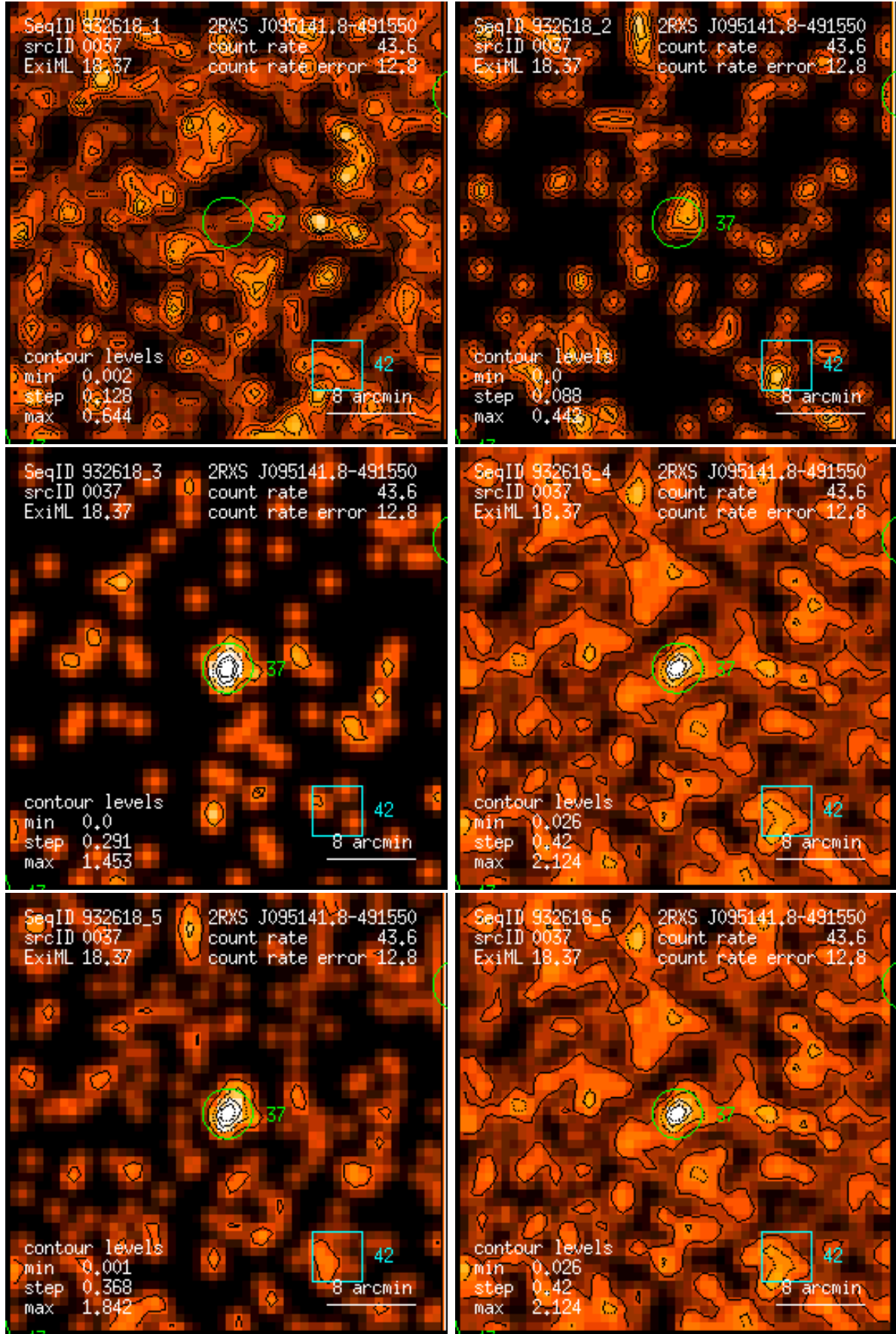
Figure 37: RASS 932618: detection 0037: band rate images, Gaussian filter: (1) PSPC channels 11 – 41, (2) 52 – 90, (3) 91 – 201, (4) 11 – 235, (5) 52 – 201, (6) 11 – 201. Broad band rates in counts/ks. Band rate contour levels in counts/ks/arcmin 2 .
