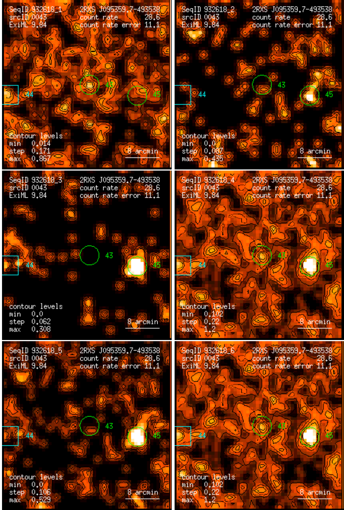
Figure 43: RASS 932618: detection 0043: band rate images, Gaussian filter: (1) PSPC channels 11 – 41, (2) 52 – 90, (3) 91 – 201, (4) 11 – 235, (5) 52 – 201, (6) 11 – 201. Broad band rates in counts/ks. Band rate contour levels in counts/ks/arcmin 2 .
