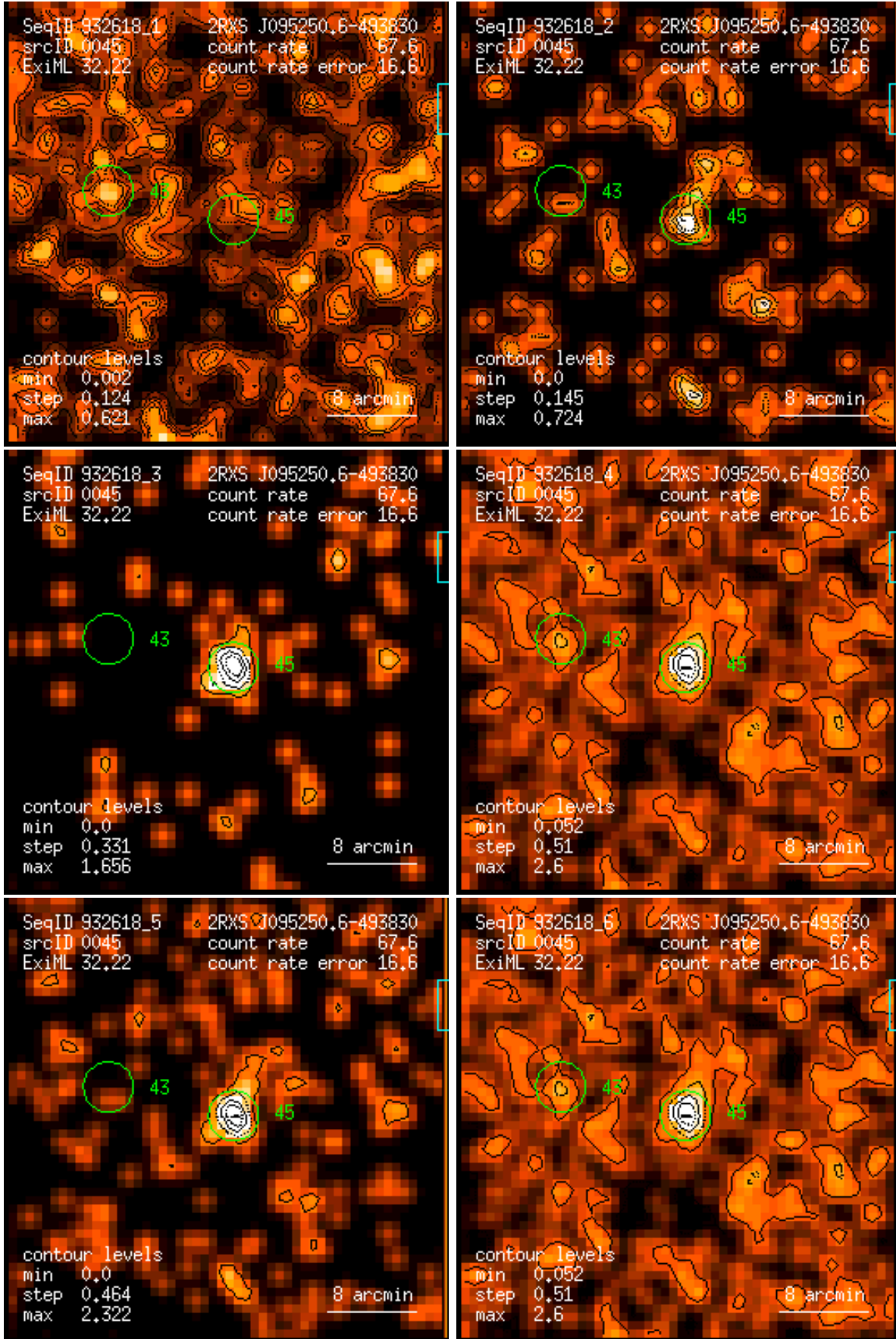
Figure 45: RASS 932618: detection 0045: band rate images, Gaussian filter: (1) PSPC channels 11 – 41, (2) 52 – 90, (3) 91 – 201, (4) 11 – 235, (5) 52 – 201, (6) 11 – 201. Broad band rates in counts/ks. Band rate contour levels in counts/ks/arcmin 2 .
