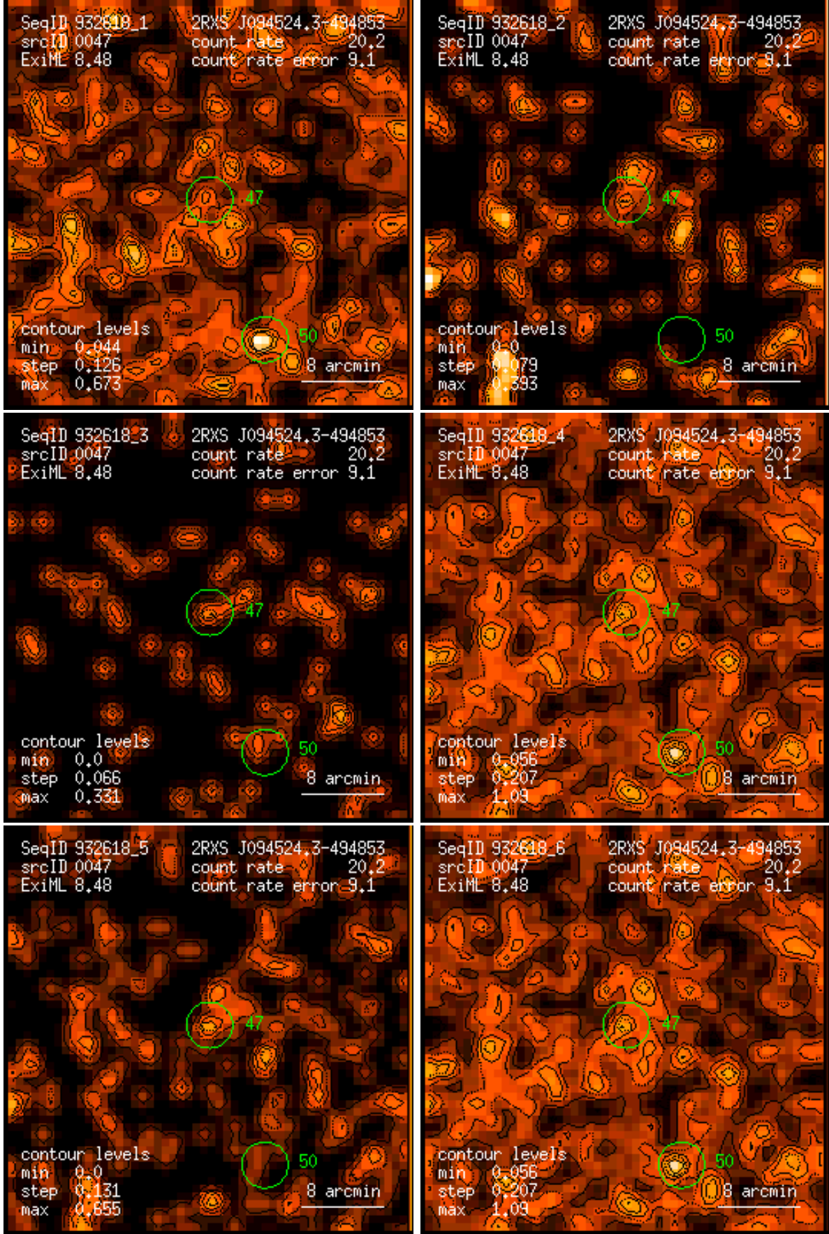
Figure 47: RASS 932618: detection 0047: band rate images, Gaussian filter: (1) PSPC channels 11 – 41, (2) 52 – 90, (3) 91 – 201, (4) 11 – 235, (5) 52 – 201, (6) 11 – 201. Broad band rates in counts/ks. Band rate contour levels in counts/ks/arcmin 2 .
