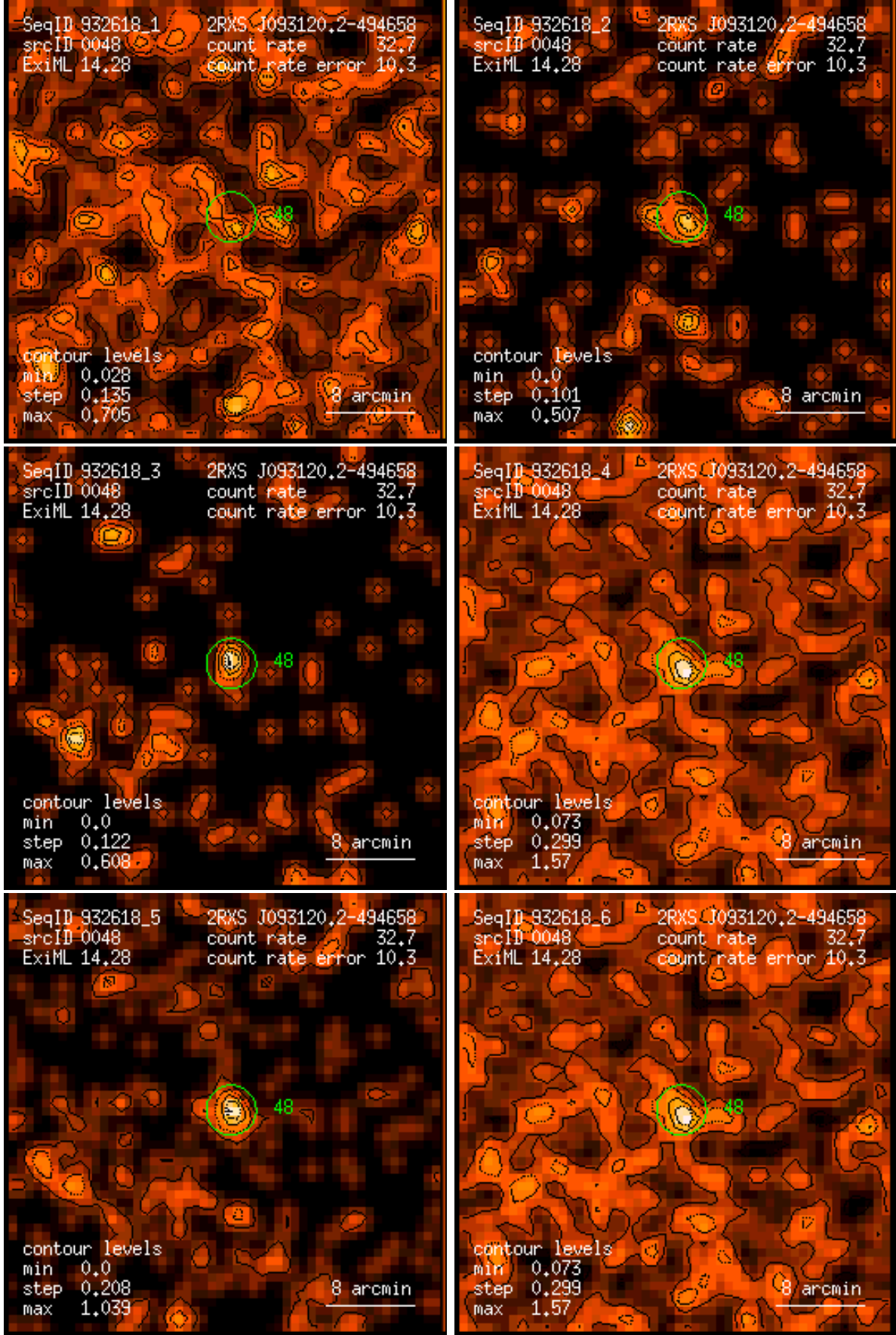
Figure 48: RASS 932618: detection 0048: band rate images, Gaussian filter: (1) PSPC channels 11 – 41, (2) 52 – 90, (3) 91 – 201, (4) 11 – 235, (5) 52 – 201, (6) 11 – 201. Broad band rates in counts/ks. Band rate contour levels in counts/ks/arcmin 2 .
