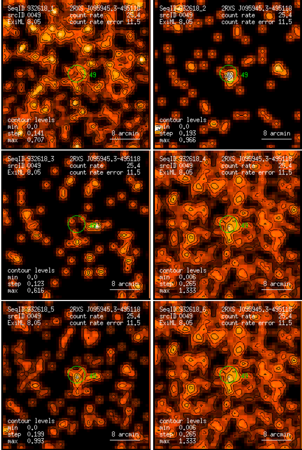
Figure 49: RASS 932618: detection 0049: band rate images, Gaussian filter: (1) PSPC channels 11 – 41, (2) 52 – 90, (3) 91 – 201, (4) 11 – 235, (5) 52 – 201, (6) 11 – 201. Broad band rates in counts/ks. Band rate contour levels in counts/ks/arcmin 2 .
