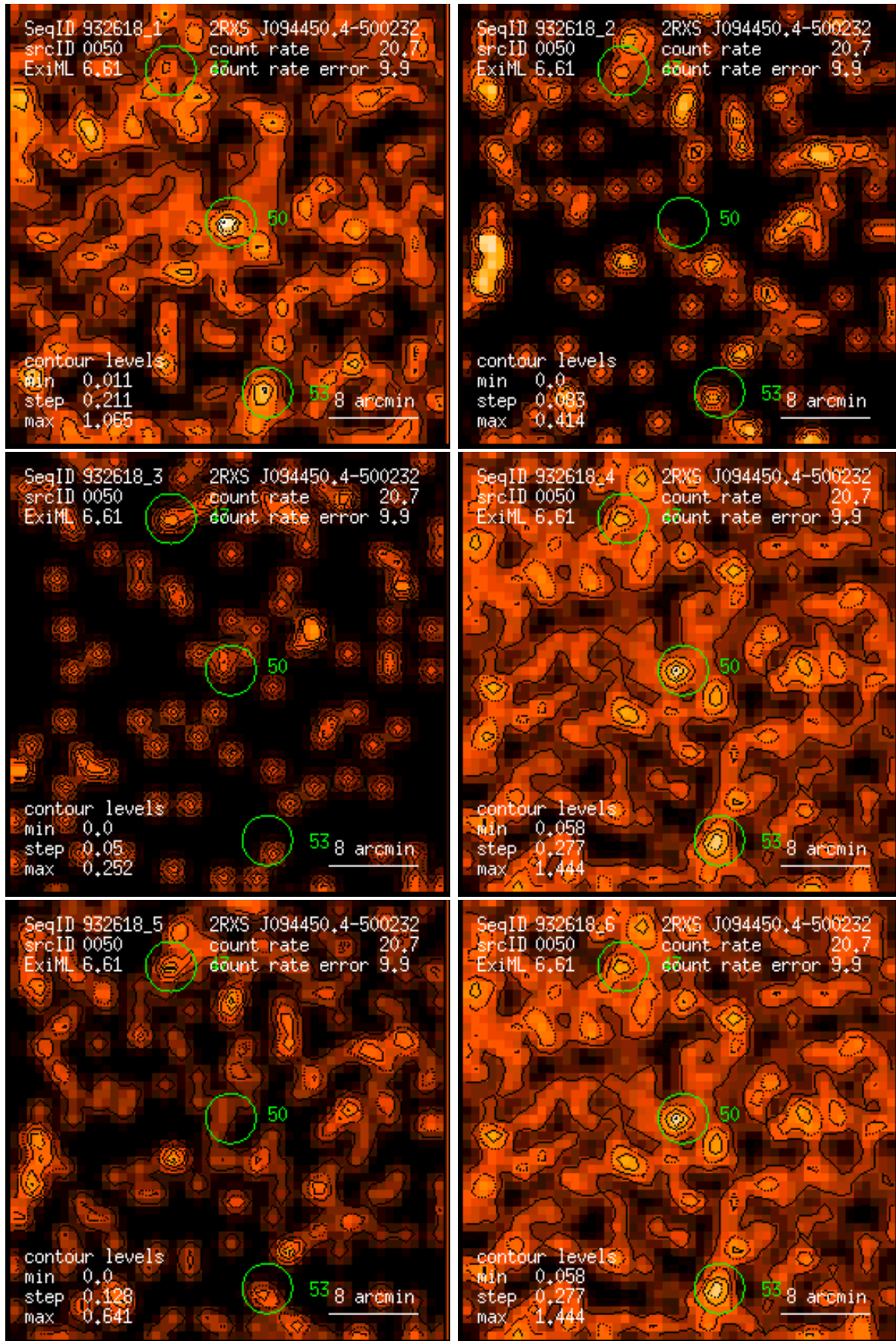
Figure 50: RASS 932618: detection 0050: band rate images, Gaussian filter: (1) PSPC channels 11 – 41, (2) 52 – 90, (3) 91 – 201, (4) 11 – 235, (5) 52 – 201, (6) 11 – 201. Broad band rates in counts/ks. Band rate contour levels in counts/ks/arcmin 2 .
