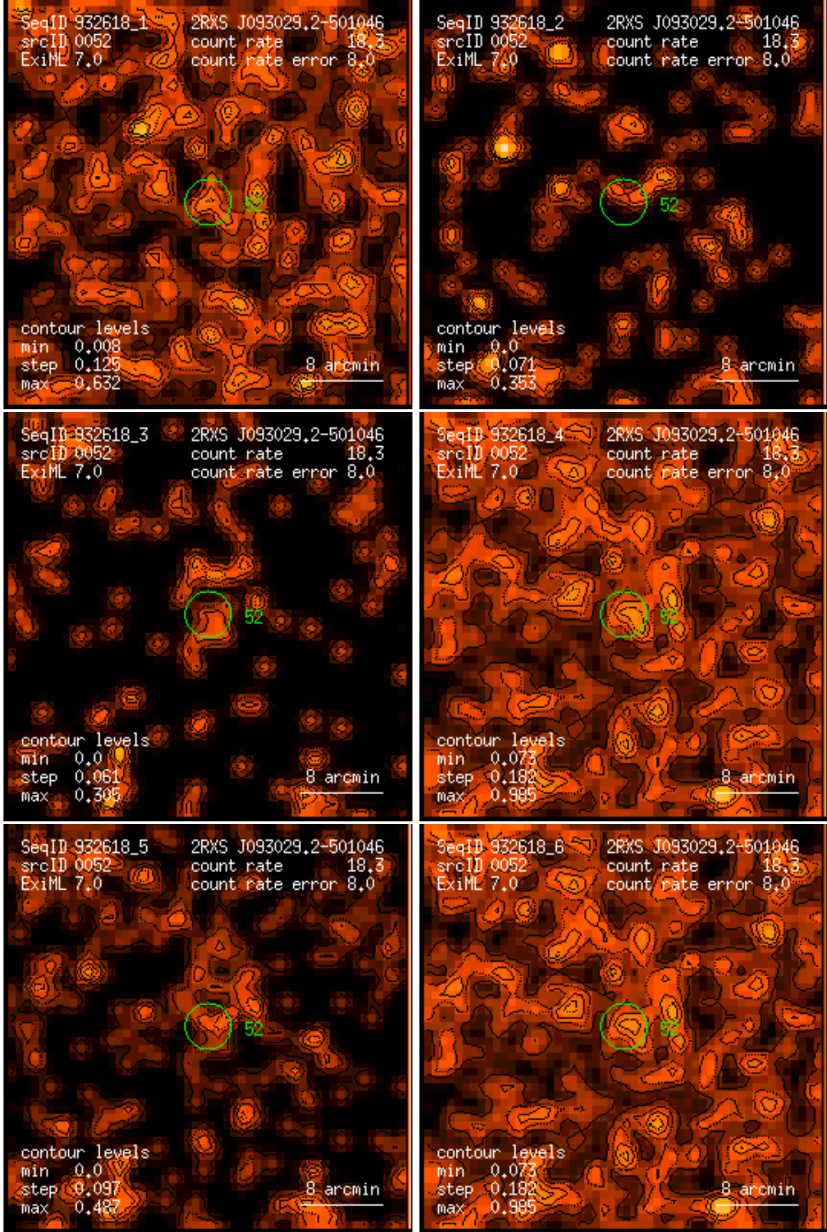
Figure 52: RASS 932618: detection 0052: band rate images, Gaussian filter: (1) PSPC channels 11 – 41, (2) 52 – 90, (3) 91 – 201, (4) 11 – 235, (5) 52 – 201, (6) 11 – 201. Broad band rates in counts/ks. Band rate contour levels in counts/ks/arcmin 2 .
