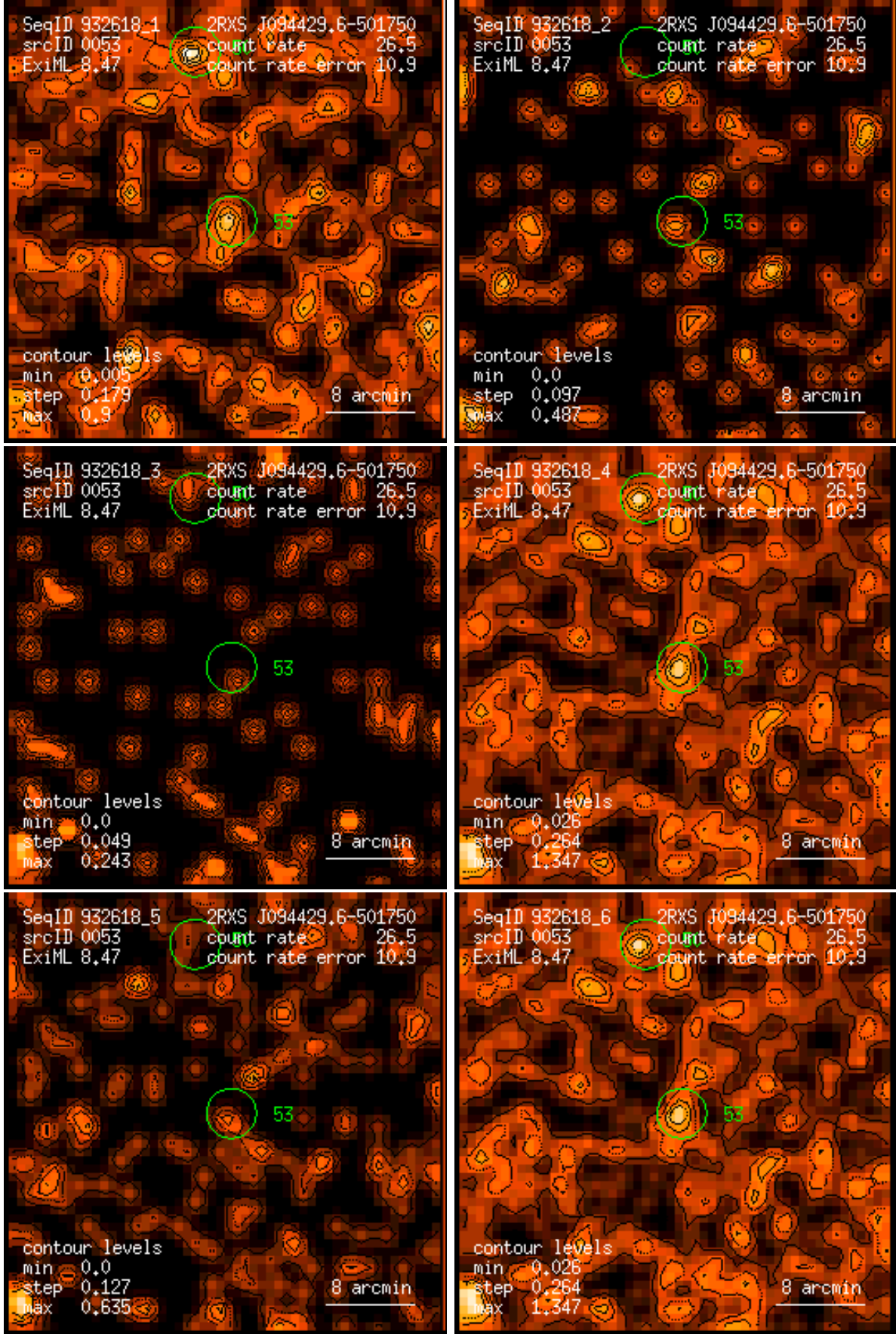
Figure 53: RASS 932618: detection 0053: band rate images, Gaussian filter: (1) PSPC channels 11 – 41, (2) 52 – 90, (3) 91 – 201, (4) 11 – 235, (5) 52 – 201, (6) 11 – 201. Broad band rates in counts/ks. Band rate contour levels in counts/ks/arcmin 2 .
