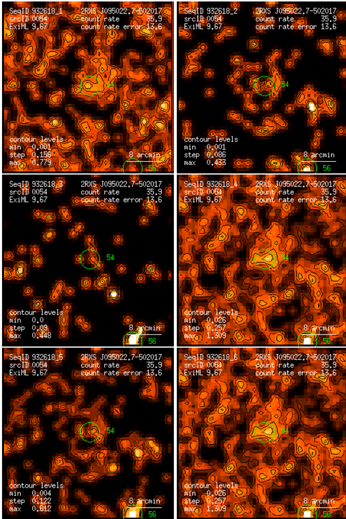
Figure 54: RASS 932618: detection 0054: band rate images, Gaussian filter: (1) PSPC channels 11 – 41, (2) 52 – 90, (3) 91 – 201, (4) 11 – 235, (5) 52 – 201, (6) 11 – 201. Broad band rates in counts/ks. Band rate contour levels in counts/ks/arcmin 2 .
