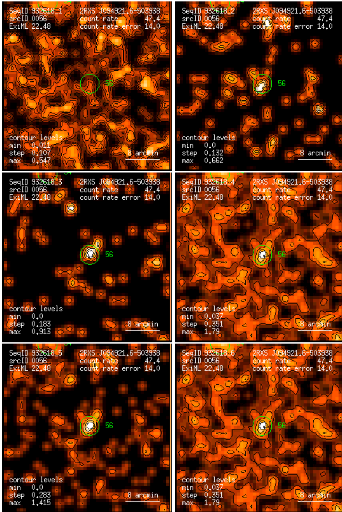
Figure 56: RASS 932618: detection 0056: band rate images, Gaussian filter: (1) PSPC channels 11 – 41, (2) 52 – 90, (3) 91 – 201, (4) 11 – 235, (5) 52 – 201, (6) 11 – 201. Broad band rates in counts/ks. Band rate contour levels in counts/ks/arcmin 2 .
