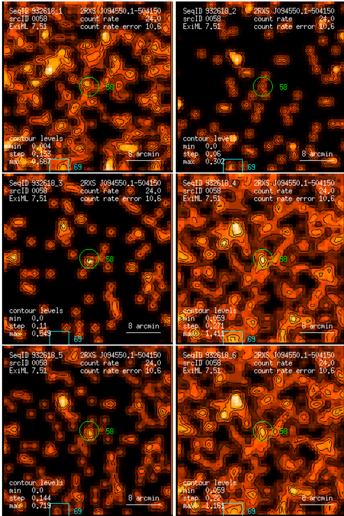
Figure 58: RASS 932618: detection 0058: band rate images, Gaussian filter: (1) PSPC channels 11 – 41, (2) 52 – 90, (3) 91 – 201, (4) 11 – 235, (5) 52 – 201, (6) 11 – 201. Broad band rates in counts/ks. Band rate contour levels in counts/ks/arcmin 2 .
