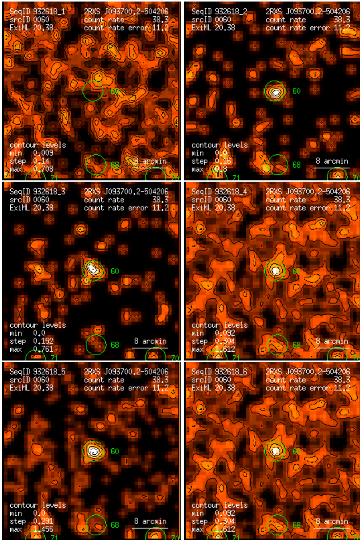
Figure 60: RASS 932618: detection 0060: band rate images, Gaussian filter: (1) PSPC channels 11 – 41, (2) 52 – 90, (3) 91 – 201, (4) 11 – 235, (5) 52 – 201, (6) 11 – 201. Broad band rates in counts/ks. Band rate contour levels in counts/ks/arcmin 2 .
