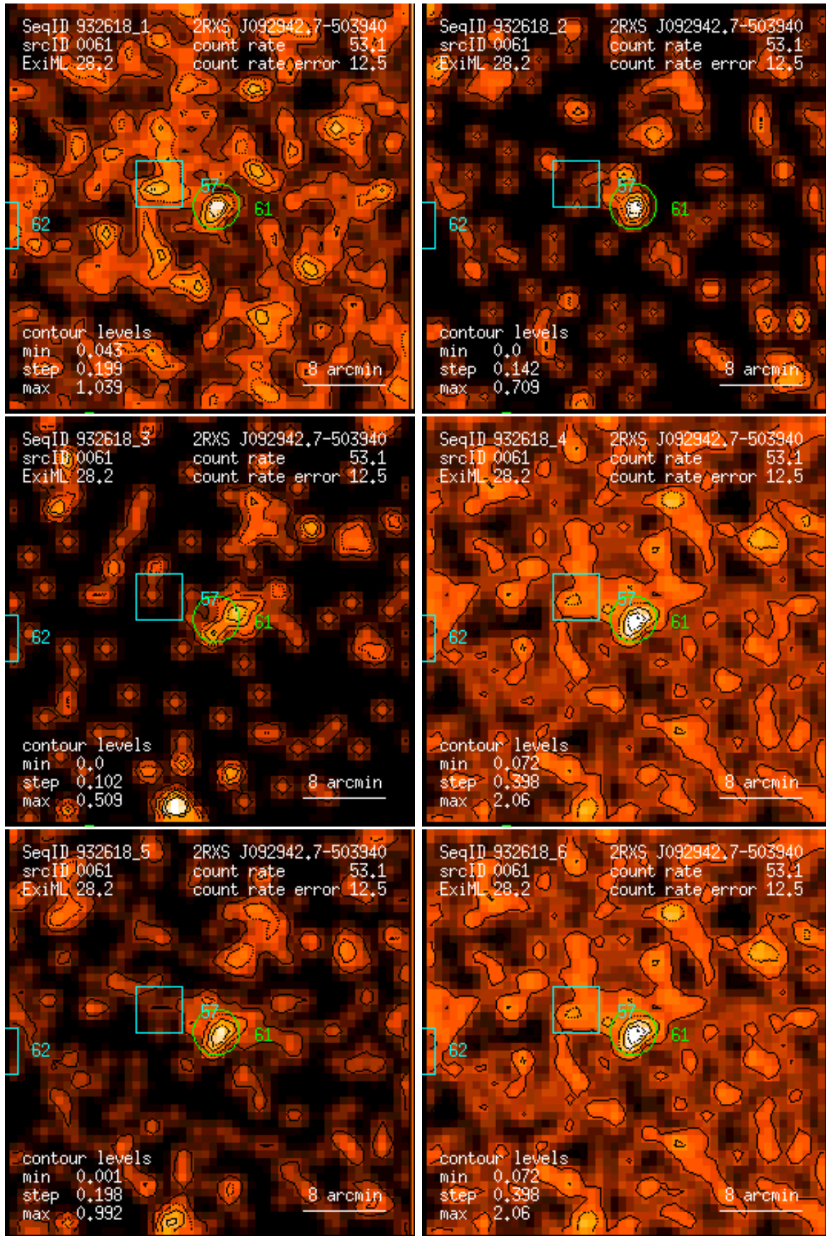
Figure 61: RASS 932618: detection 0061: band rate images, Gaussian filter: (1) PSPC channels 11 – 41, (2) 52 – 90, (3) 91 – 201, (4) 11 – 235, (5) 52 – 201, (6) 11 – 201. Broad band rates in counts/ks. Band rate contour levels in counts/ks/arcmin 2 .
