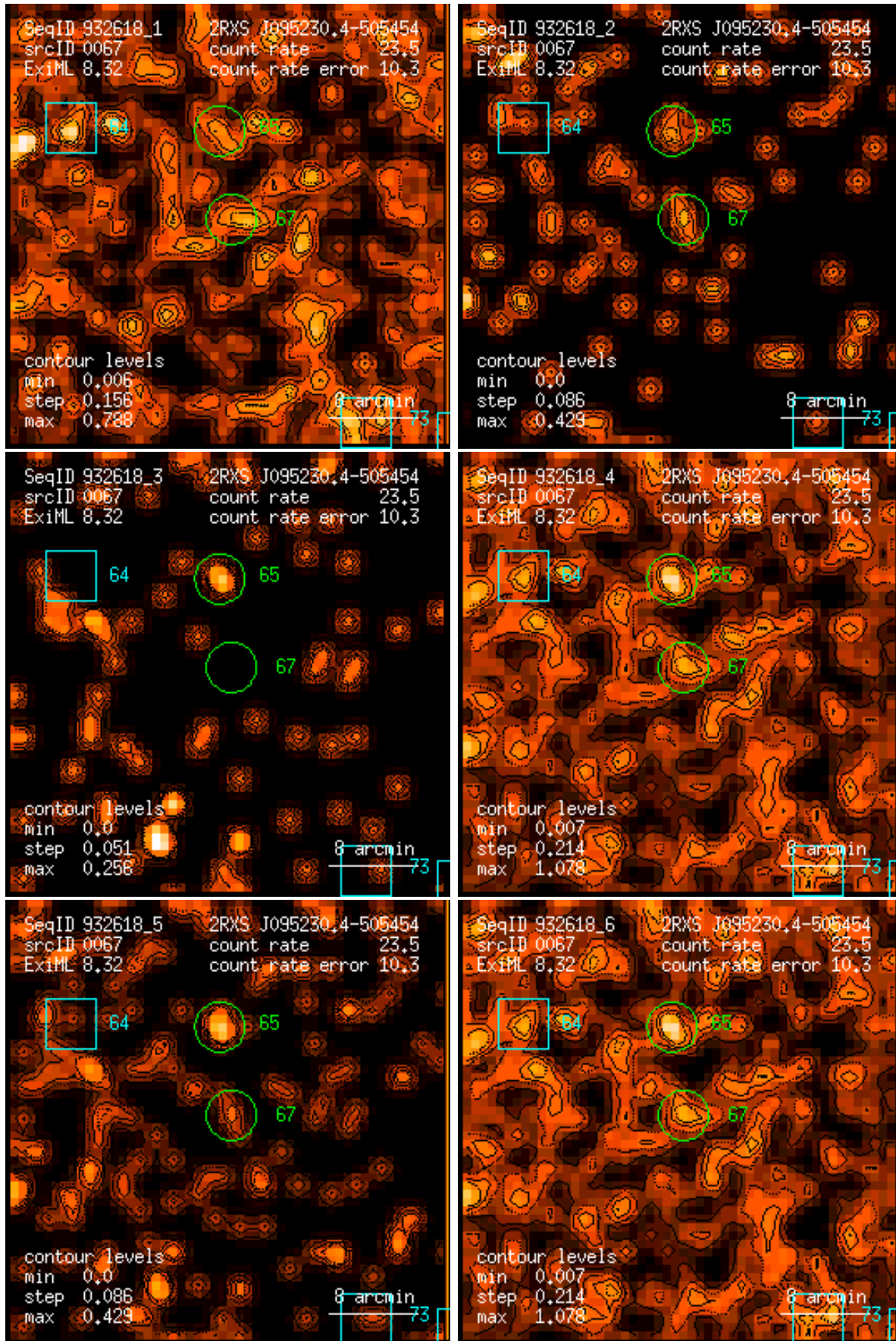
Figure 67: RASS 932618: detection 0067: band rate images, Gaussian filter: (1) PSPC channels 11 – 41, (2) 52 – 90, (3) 91 – 201, (4) 11 – 235, (5) 52 – 201, (6) 11 – 201. Broad band rates in counts/ks. Band rate contour levels in counts/ks/arcmin 2 .
