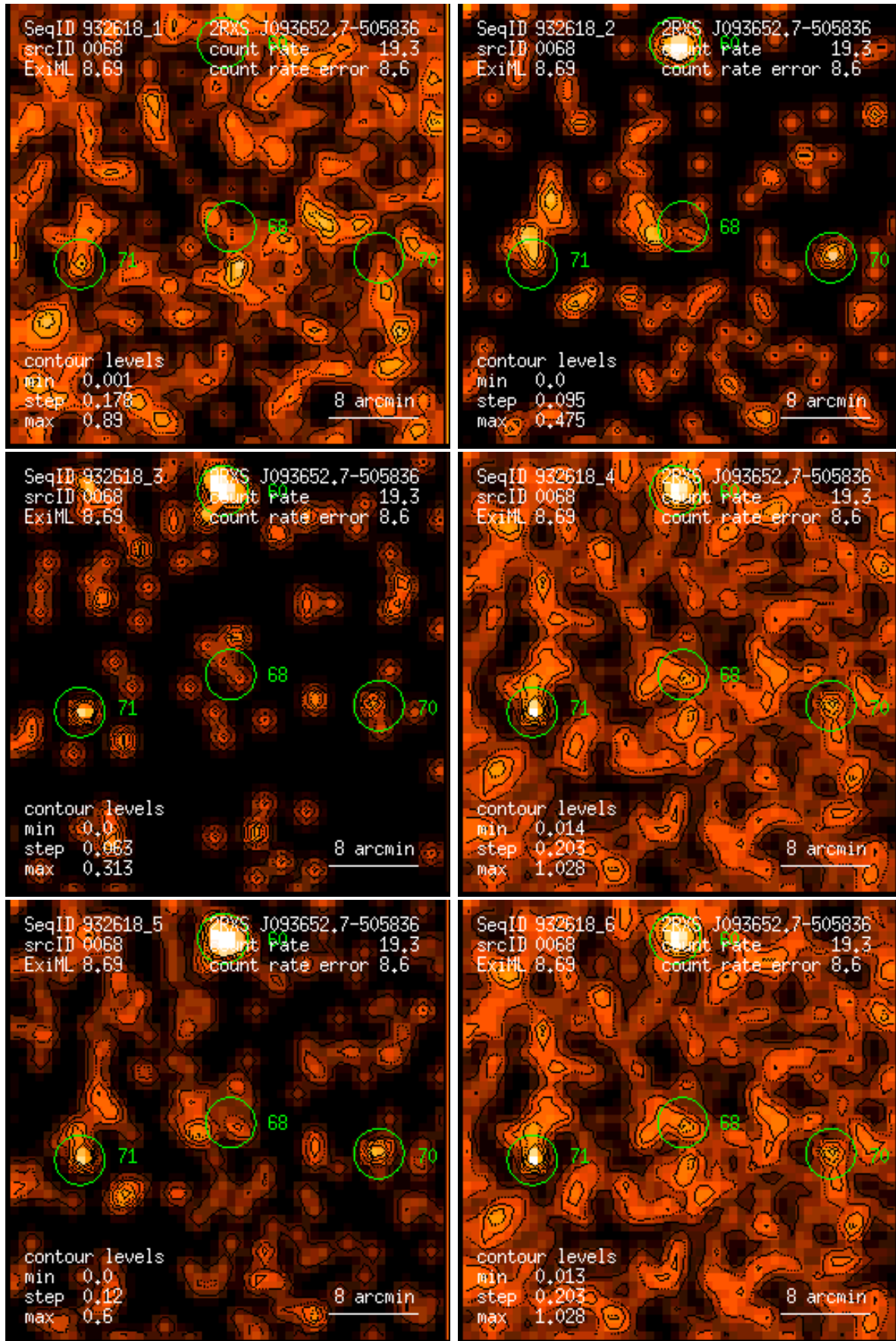
Figure 68: RASS 932618: detection 0068: band rate images, Gaussian filter: (1) PSPC channels 11 – 41, (2) 52 – 90, (3) 91 – 201, (4) 11 – 235, (5) 52 – 201, (6) 11 – 201. Broad band rates in counts/ks. Band rate contour levels in counts/ks/arcmin 2 .
