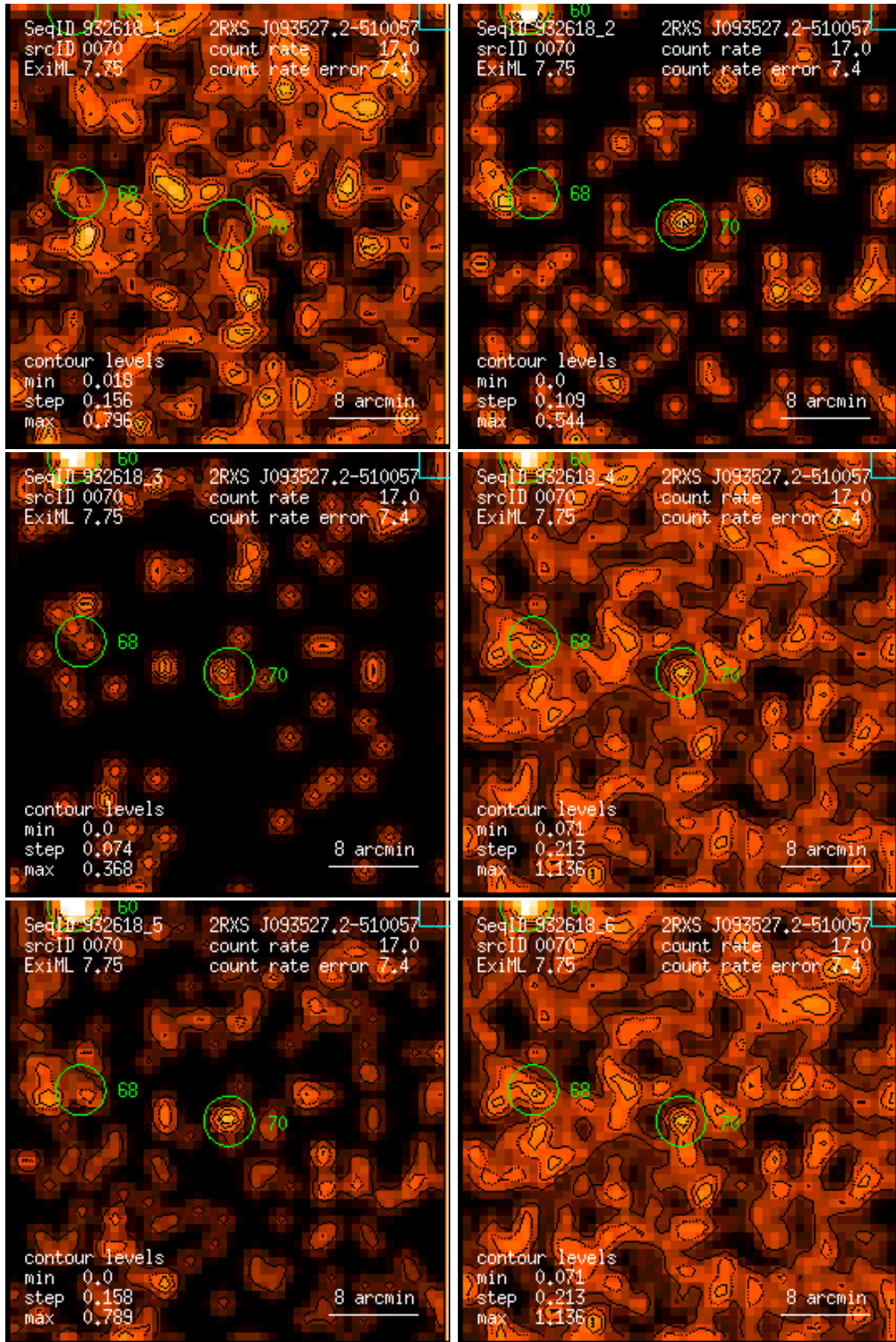
Figure 70: RASS 932618: detection 0070: band rate images, Gaussian filter: (1) PSPC channels 11 – 41, (2) 52 – 90, (3) 91 – 201, (4) 11 – 235, (5) 52 – 201, (6) 11 – 201. Broad band rates in counts/ks. Band rate contour levels in counts/ks/arcmin 2 .
