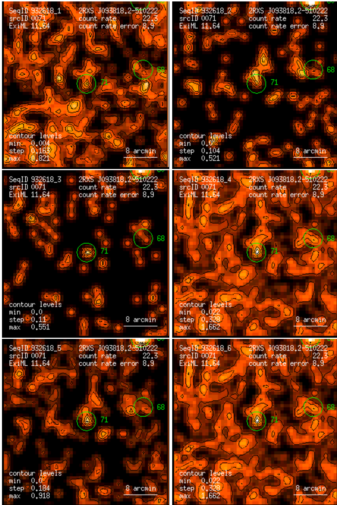
Figure 71: RASS 932618: detection 0071: band rate images, Gaussian filter: (1) PSPC channels 11 – 41, (2) 52 – 90, (3) 91 – 201, (4) 11 – 235, (5) 52 – 201, (6) 11 – 201. Broad band rates in counts/ks. Band rate contour levels in counts/ks/arcmin 2 .
