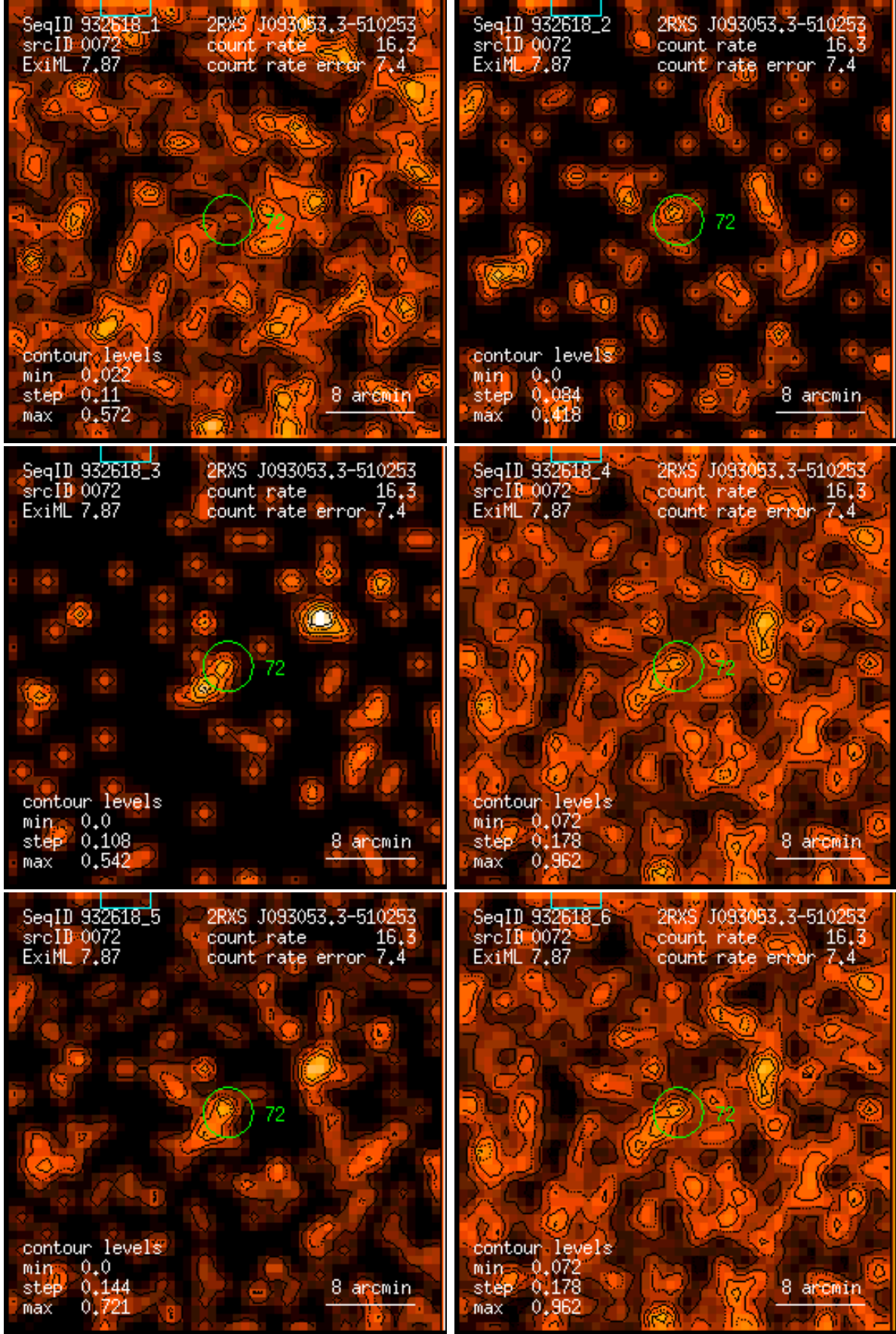
Figure 72: RASS 932618: detection 0072: band rate images, Gaussian filter: (1) PSPC channels 11 – 41, (2) 52 – 90, (3) 91 – 201, (4) 11 – 235, (5) 52 – 201, (6) 11 – 201. Broad band rates in counts/ks. Band rate contour levels in counts/ks/arcmin 2 .
