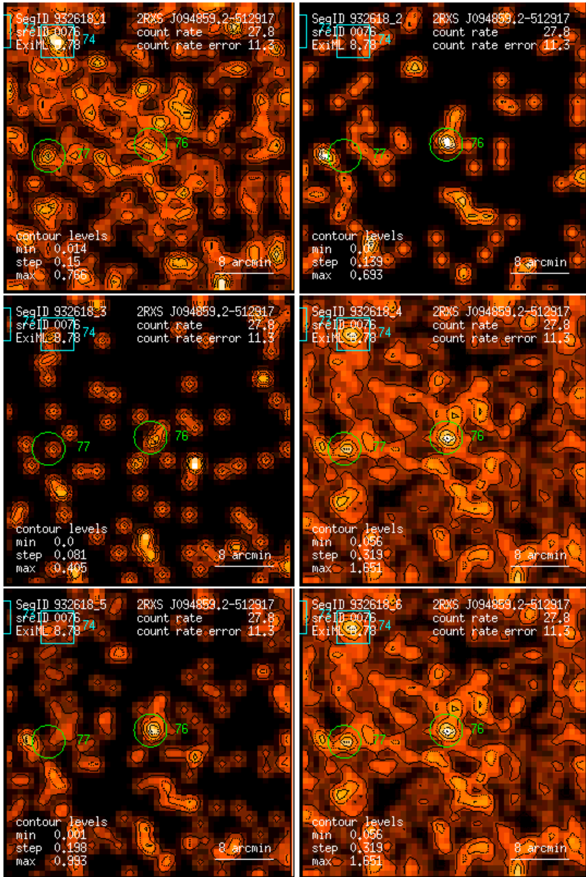
Figure 76: RASS 932618: detection 0076: band rate images, Gaussian filter: (1) PSPC channels 11 – 41, (2) 52 – 90, (3) 91 – 201, (4) 11 – 235, (5) 52 – 201, (6) 11 – 201. Broad band rates in counts/ks. Band rate contour levels in counts/ks/arcmin 2 .
