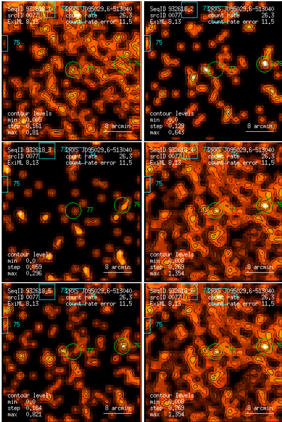
Figure 77: RASS 932618: detection 0077: band rate images, Gaussian filter: (1) PSPC channels 11 – 41, (2) 52 – 90, (3) 91 – 201, (4) 11 – 235, (5) 52 – 201, (6) 11 – 201. Broad band rates in counts/ks. Band rate contour levels in counts/ks/arcmin 2 .
